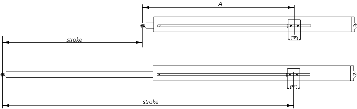
Fig.102 - Dimensions of type G spindle actuator with shifted pivot point A - dimension depends on opening angle and height of the window
