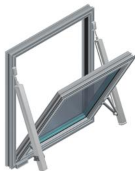
Fig.53 - mcr OSO THERM 75 smoke exhaust window with two G spindle actuators with shifted pivot point
