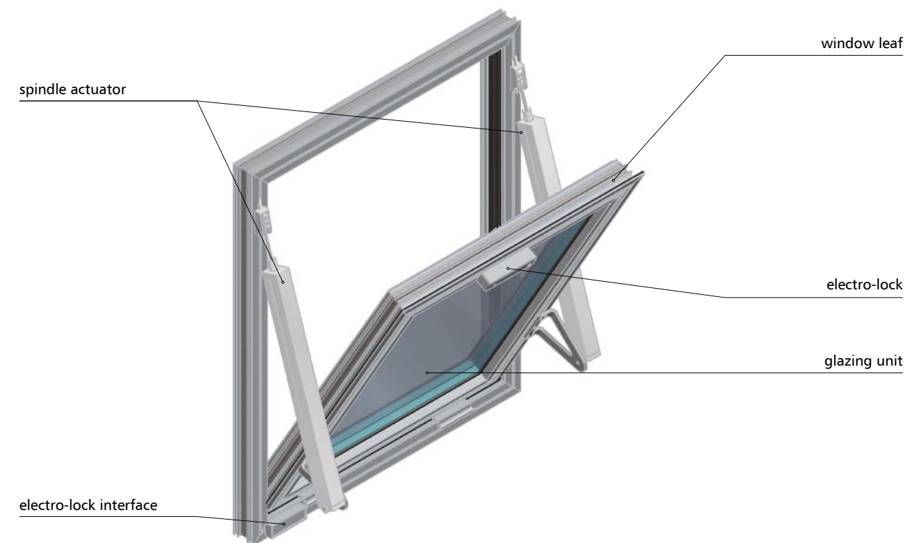
Fig.62 - mcr OSO THERM 75 smoke exhaust window opening inwards by means of two G spindle actuators with electro-lock and interface
