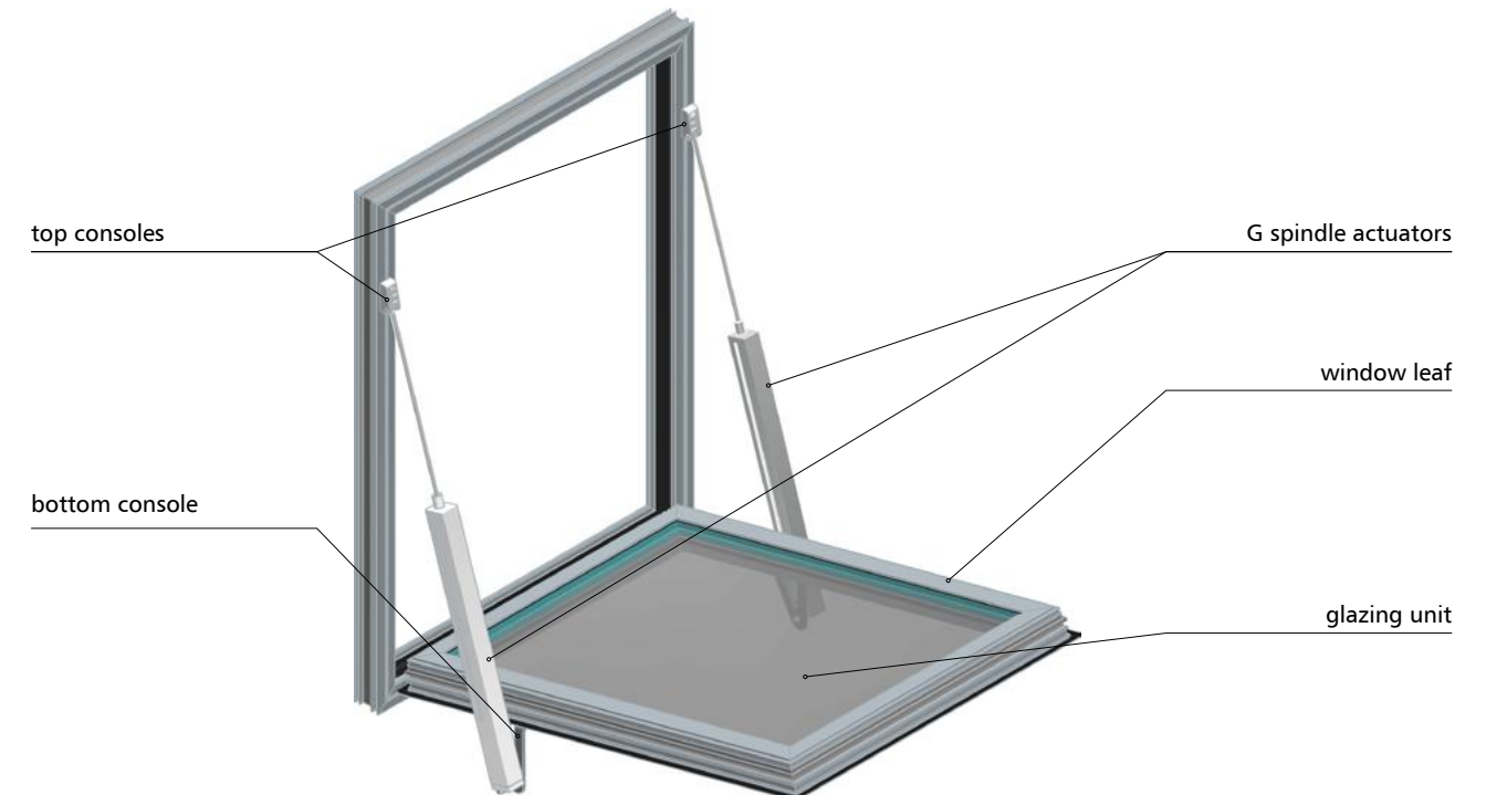
Fig.61 - mcr OSO THERM 75 smoke exhaust window opening inwards by means of two spindle actuators
