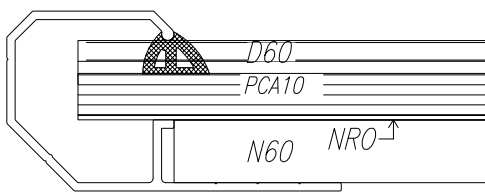
Fig.111 Skylight section; glazing - single multi-chamber polycarbonate panel and NRO panel
