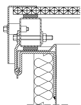
Fig.33 Vent section, glazing: structured multi-chamber polycarbonate panel
