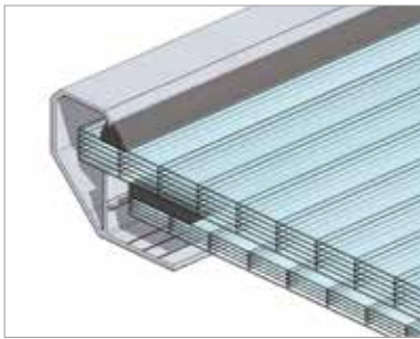
Fig.106 Skylight glazing – two multi-chamber polycarbonate panels (PCA16 + PCA10) with air gap between (PP)
