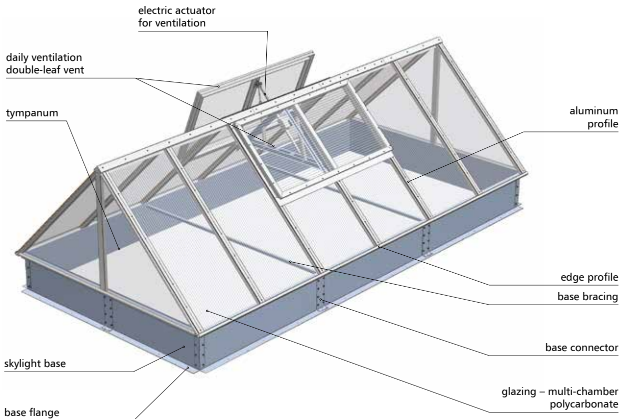
Fig. 79 Design of mcr PROLIGHT triangular shaped continuous rooflight with double-leaf vent, with electric actuator for daily ventilation
