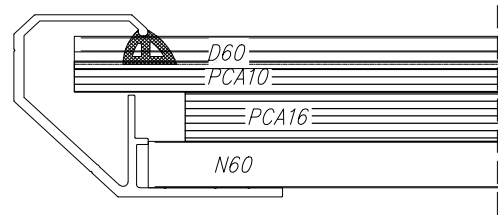
Fig.100 Section of skylight of width 1.5÷4.0 m; supporting profile (N) and pressing profile (D) of width 60 mm
