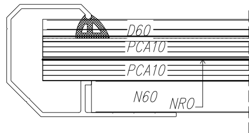
Fig.120 Section of skylight of width 1.2÷3.5 m; supporting profile (N) and pressing profile (D) of width 60 mm
