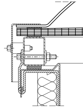
Fig.51 Vent section, glazing B roof (t1)
