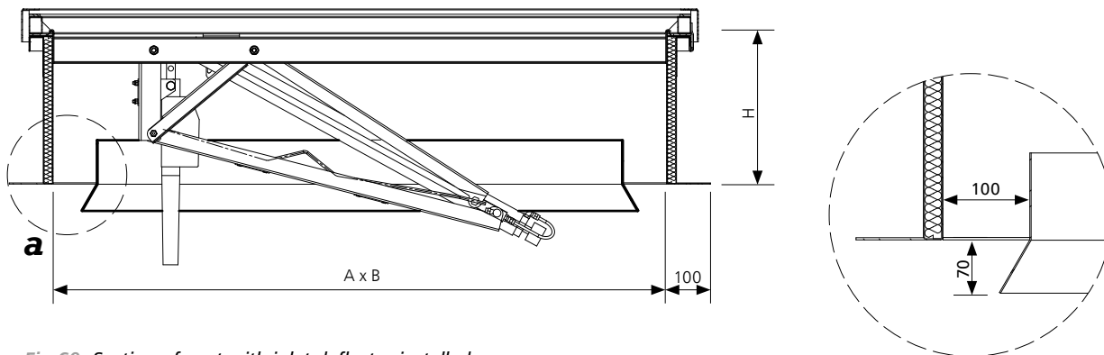
Fig.60 Section of vent with inlet deflector installed
