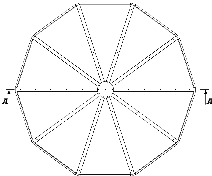
Fig.93 Top view of mcr PROLIGHT igloo skylight
