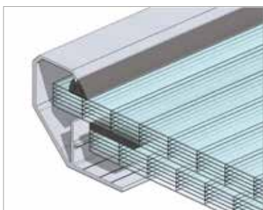
Fig.108 Skylight glazing – two multi-chamber polycarbonate panels (PCA16 + PCA16) with air gap between (PP)
