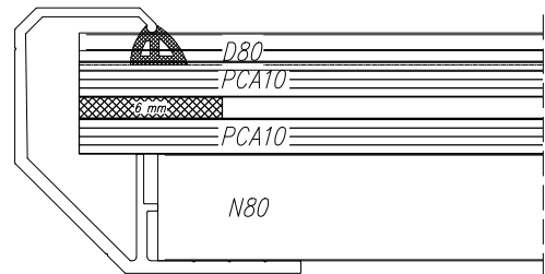
Fig.105 Section of skylight of width 3.5÷4.0 m; supporting profile (N) and pressing profile (D) of width 80 mm
