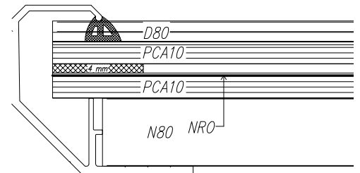
Fig.123 Skylight glazing – multi-chamber polycarbonate panel (PCA), NRO panel
