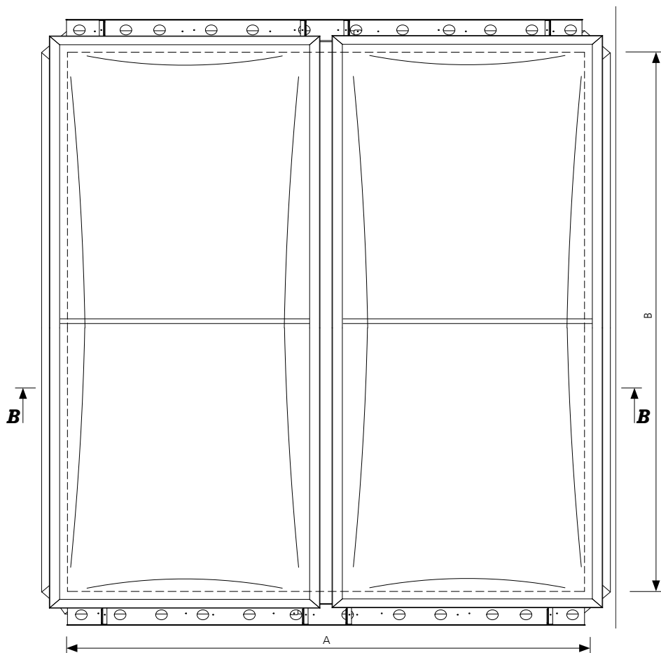
Fig.6 Top view of mcr PROLIGHT DVP smoke vent in closed position, dimensions in [mm]
