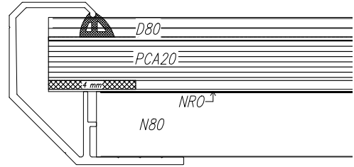
Fig.118 Section of skylight of width 1.5÷4.0 m; supporting profile (N) and pressing profile (D) of width 60 mm
