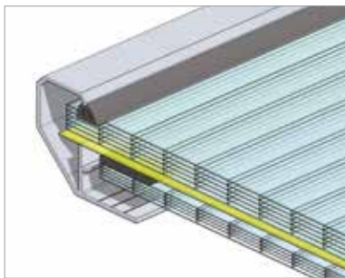
Fig.124 Skylight glazing: two multi-chamber polycarbonate panels (PCA16+PCA10) with NRO panel and air gap (PP) between
