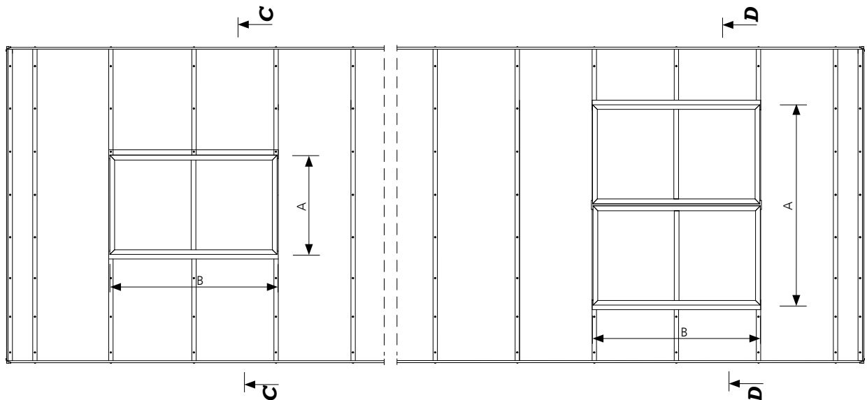
Fig.78 Top view of mcr PROLIGHT arch shaped continuous rooflight with integrated smoke exhaust and daily ventilation single and double-leaf vent
