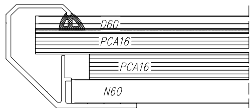
Fig.102 Section of skylight of width 1.5÷6.0 m; supporting profile (N) and pressing profile (D) of width 60 mm
