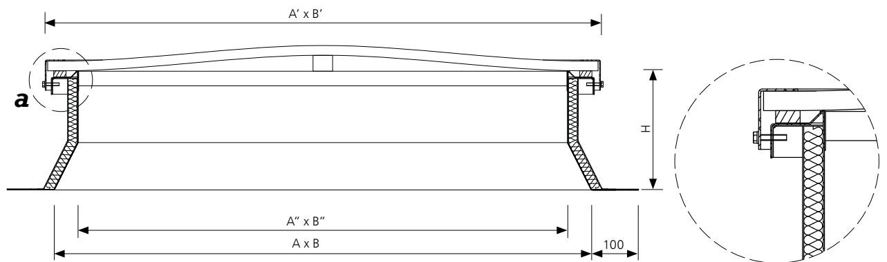
Fig.17 Section B-B of mcr PROLIGHT NG-A fixed skylight, dimensions in [mm]
