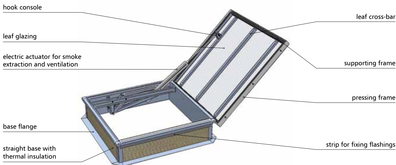
Fig.52 mcr PROLIGHT C100 smoke vent with roof access function and electric control for smoke extraction and ventilation
