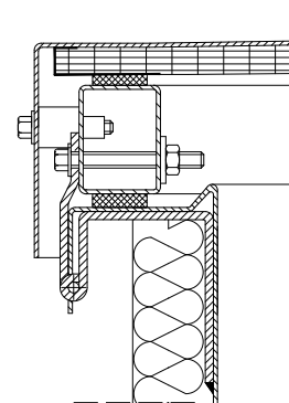
Fig.45 Vent section, glazing – ALU envelope cover with multi-chamber polycarbonate
