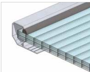
Fig.96 Skylight glazing – two multi-chamber polycarbonate panels (PCA10 + PCA10)
