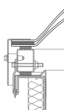
Fig.35 Vent section, glazing: double-layer acrylic dome
