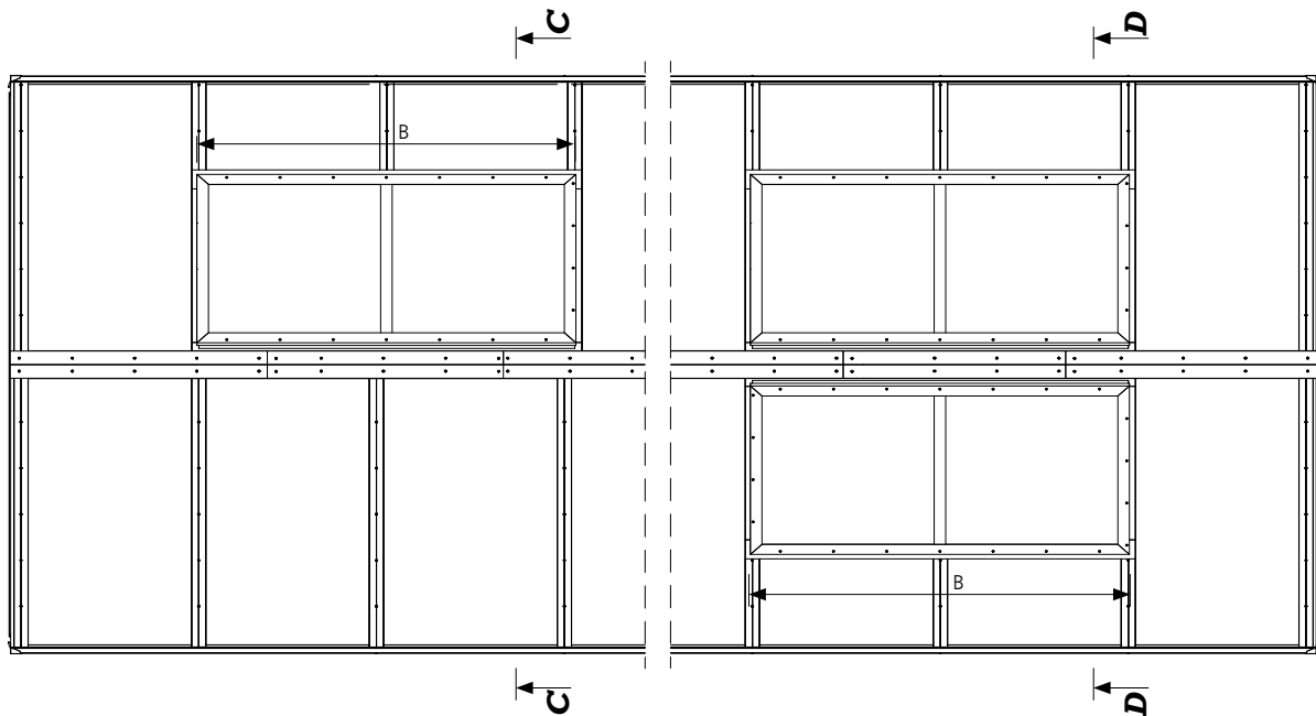
Fig.85 Top view of mcr PROLIGHT triangular shaped continuous rooflight with daily ventilation single-leaf and double-leaf vent
