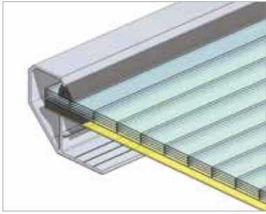
Fig.112 Skylight glazing: multi-chamber polycarbonate panel (PCA10), NRO panel with air gap between (PP)
