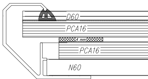
Fig.109 Section of skylight of width 1.5÷4.0 m; supporting profile (N) and pressing profile (D) of width 60 mm
