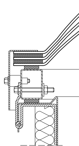
Fig.41 Vent section, glazing: triple-layer solid polycarbonate dome
