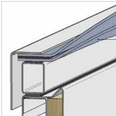
Fig.34 Vent glazing – double-layer acrylic dome
