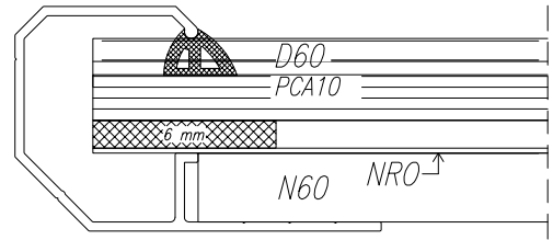
Fig.113 Section of skylight of width 1.5÷4.0 m; supporting profile (N) and pressing profile (D) of width 60 mm
