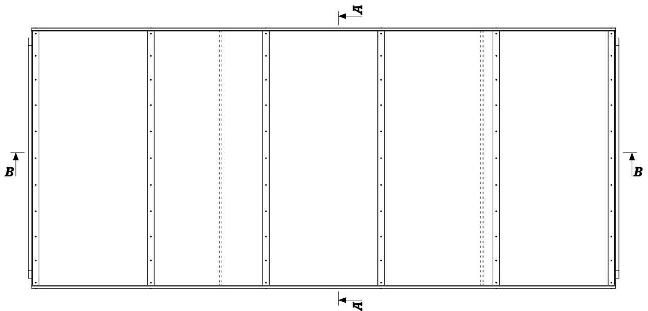
Fig.74 Top view of mcr PROLIGHT continuous rooflight
