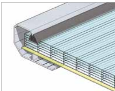
Fig.110 Skylight glazing – multi-chamber polycarbonate panel (PCA), NRO panel
