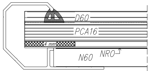
Fig.116 Section of skylight of width 1.5÷4.0 m; supporting profile (N) and pressing profile (D) of width 60 mm
