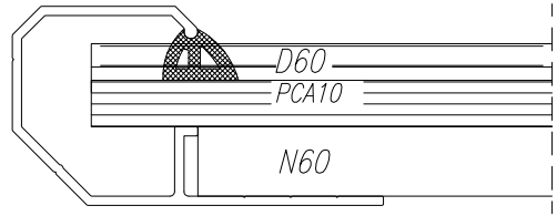
Fig.95 Skylight section; glazing: single multi-chamber polycarbonate panel
