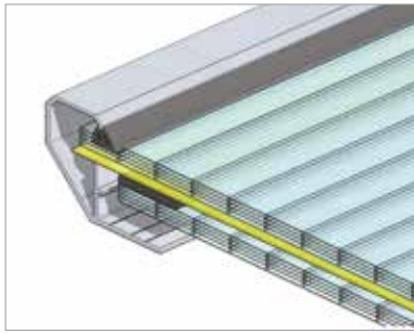
Fig.121 Skylight glazing: two multi-chamber polycarbonate panels (PCA10+PCA10) with air gap (PP) and NRO panel between
