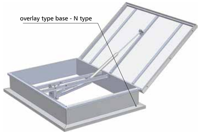
Fig.65 mcr PROLIGHT E type smoke vent with N type base
