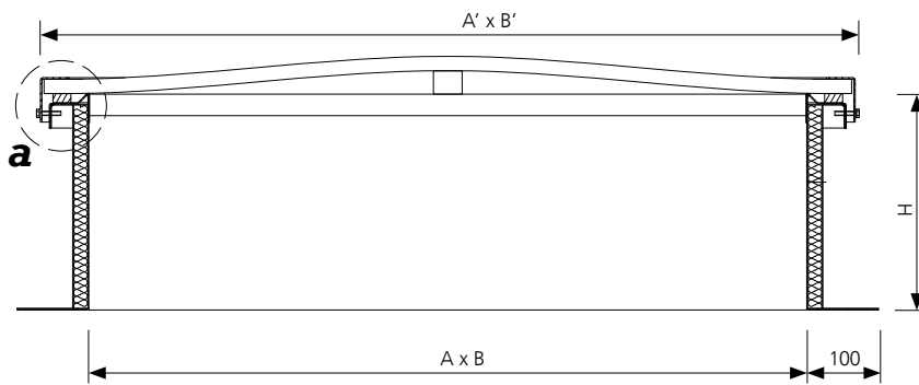
Fig.14 Section B-B of mcr PROLIGHT C or E fixed skylight, dimensions in [mm]
