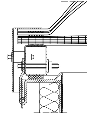
Fig.49 Vent section, glazing – acrylic dome or solid polycarbonate dome and multi-chamber polycarbonate panel
