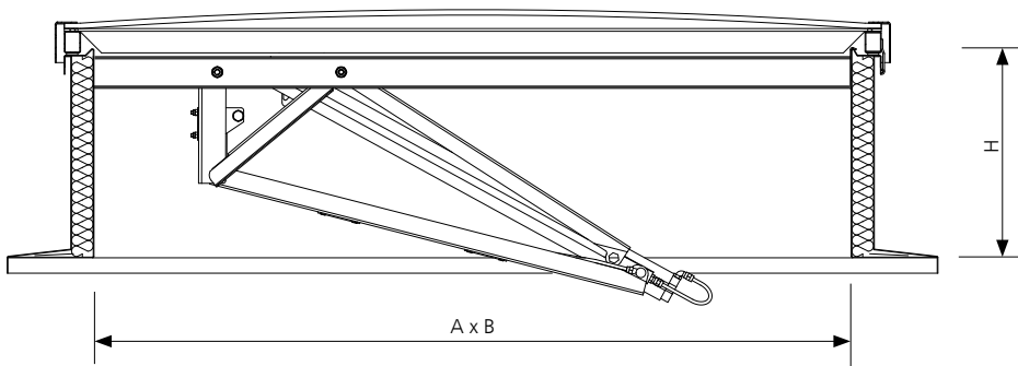
Fig.66 Section of mcr PROLIGHT E type vent with N plinth type base
