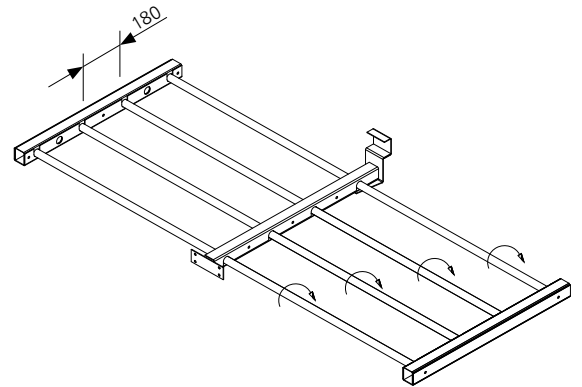
Fig.62 Anti-burglar grid for smoke vent
