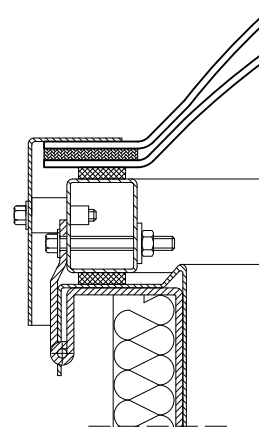
Fig.39 Vent section, glazing: double-layer solid polycarbonate dome
