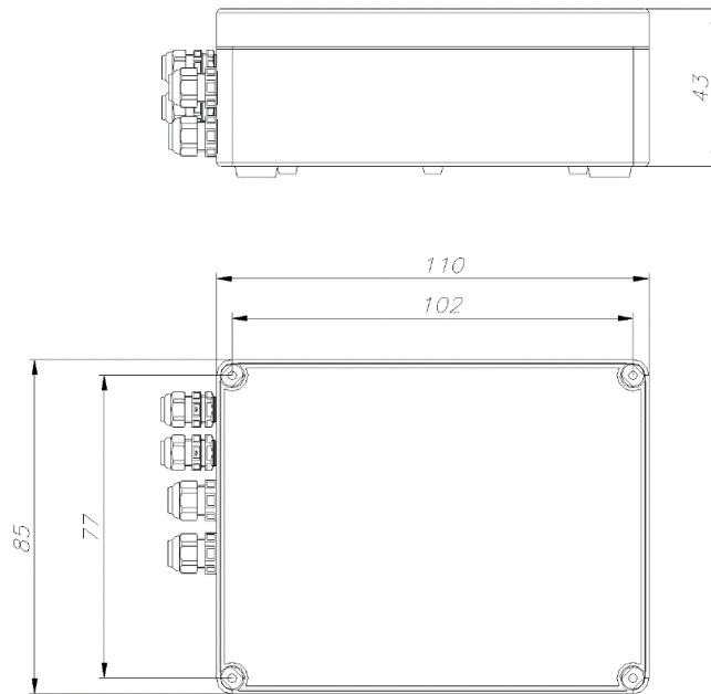
Figure 107 Dimensions of mcr SEP network separator installation holes.
