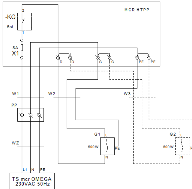
Figure 37 Internal HT system connections circuit diagram.
