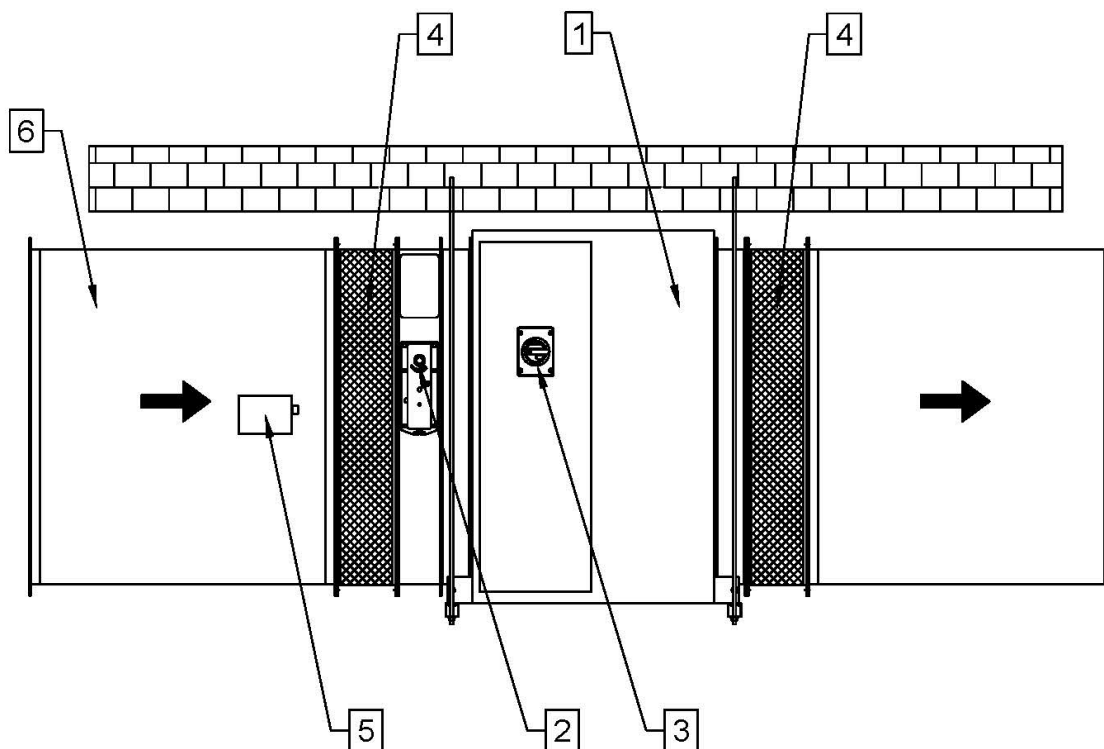
Figure 6 Sample installation of an air supply kit for the mcr EXi-F system in the duct version: 1 - fan, 2 - damper with actuator, 3 - service disconnect or connection box, 4 - flexible connection, 5 duct smoke detector.
