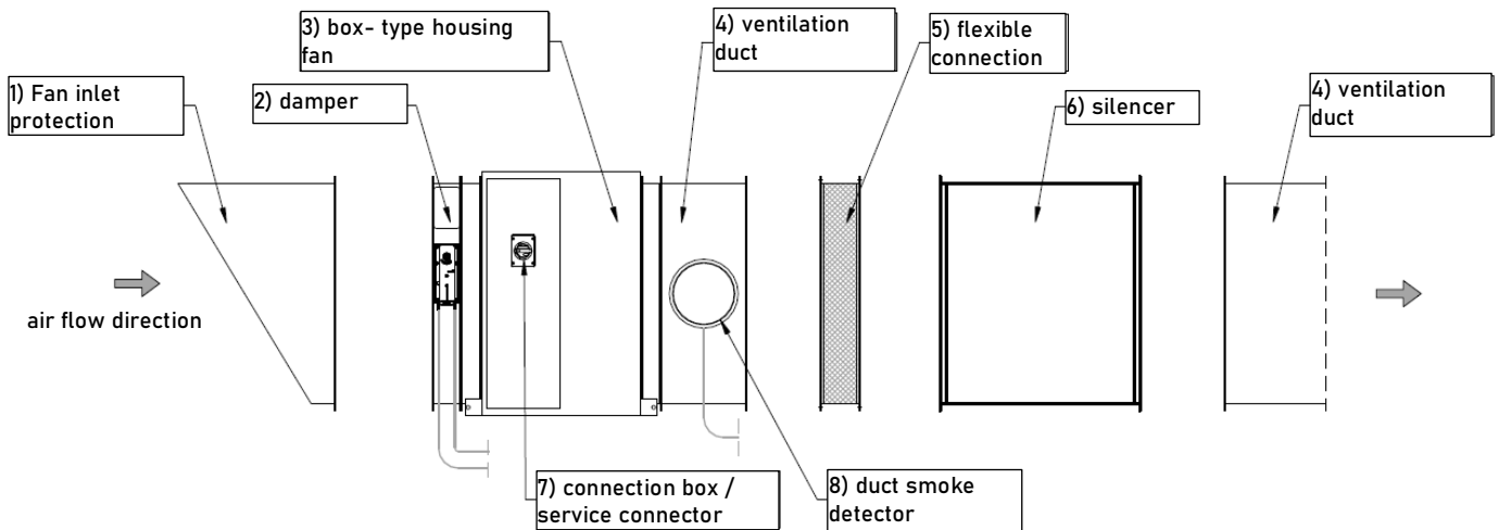
Figure 95 Sample standard horizontal installation of a set of mcr EXi-F system components: 1 - fan inlet protection, 2 - damper, 3 - mcr Monsun E1 fan in a box-type housing 4 - ventilation duct (pipe), 5 - flexible connection, 6 - silencer, 7 - connection box / service connector, 8 - duct smoke detector.
