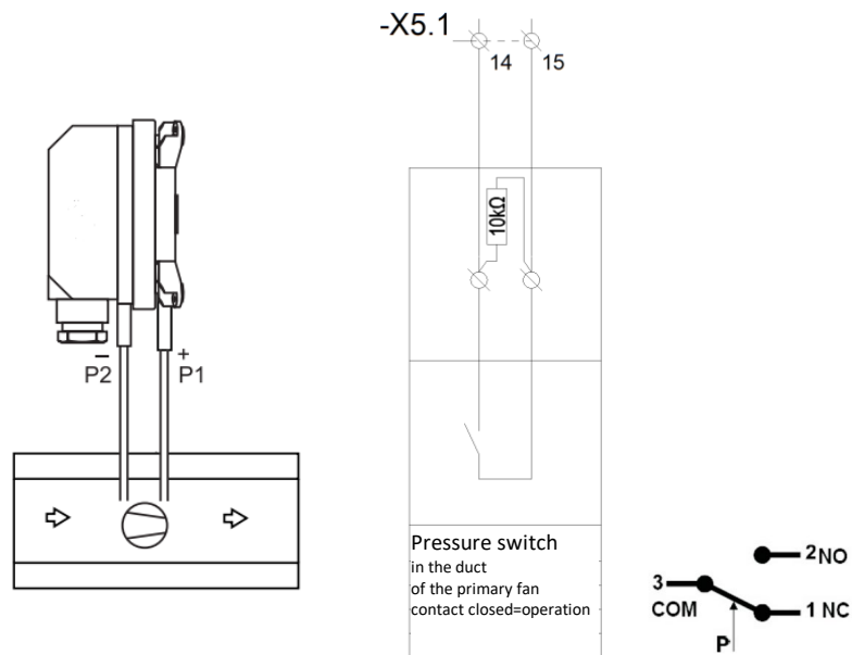
Figure 44 Electrical diagram of a LF or DW series differential pressure switch.
