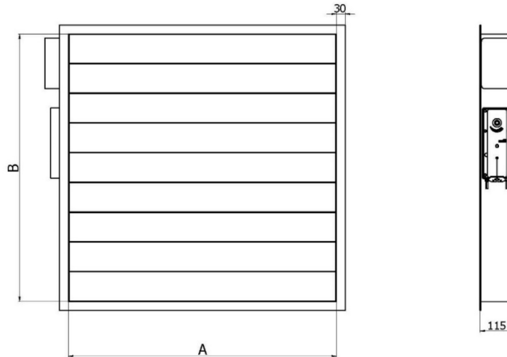
Figure 13 Overview of a shut-off damper.
