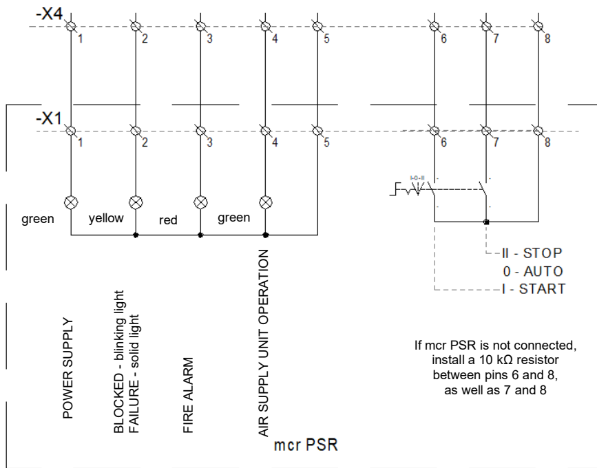
Figure 81 mcr PSR manual control panel connections circuit diagram.
