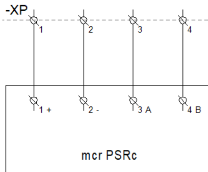
Figure 82 mcr PSRC manual control panel connections circuit diagram.
