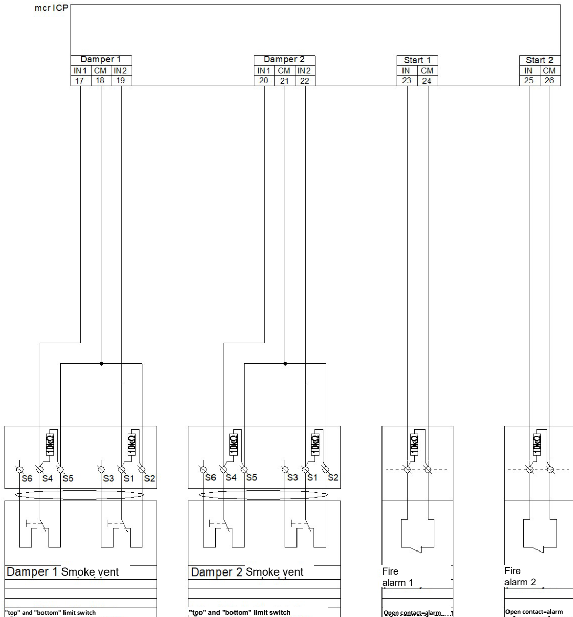
Figure 79 Connection diagram for fire ventilation vent limit switches and SSP alarms.
