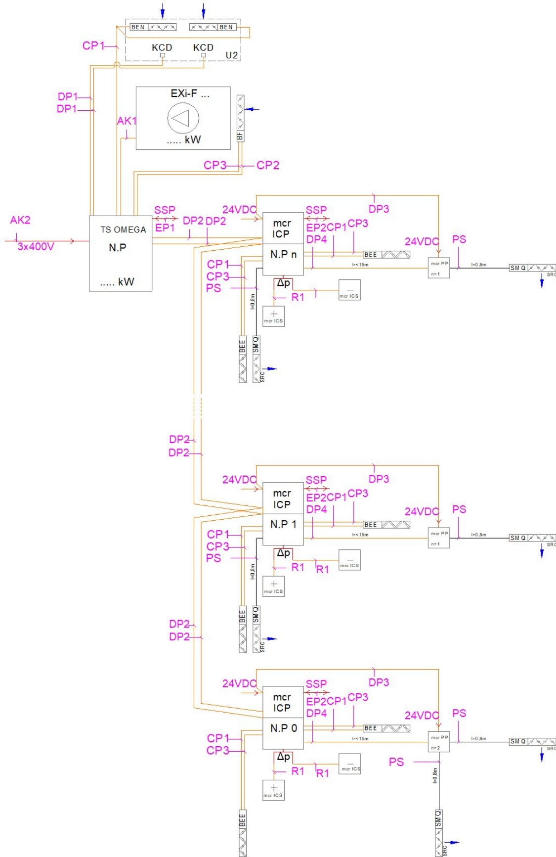
Figure 56 Schematic wiring diagram for a unit with high-speed mcr ICP dampers secured with smoke control system vents located at a higher distance from the regulator, using an mcr PP box.
