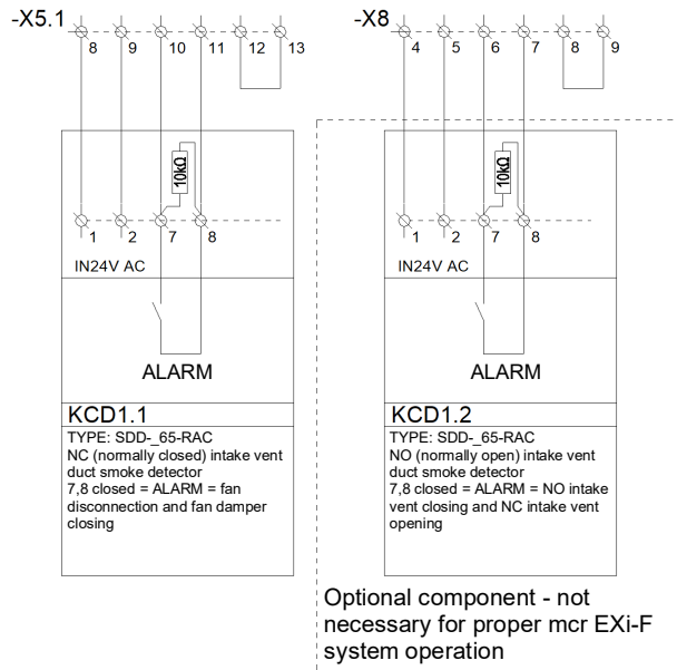
Figure 85 SDD-65-RAC duct smoke detector connections circuit diagram.
