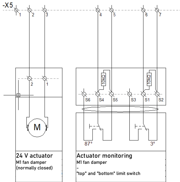
Figure 66 Shut-off damper actuator connections circuit diagram.
