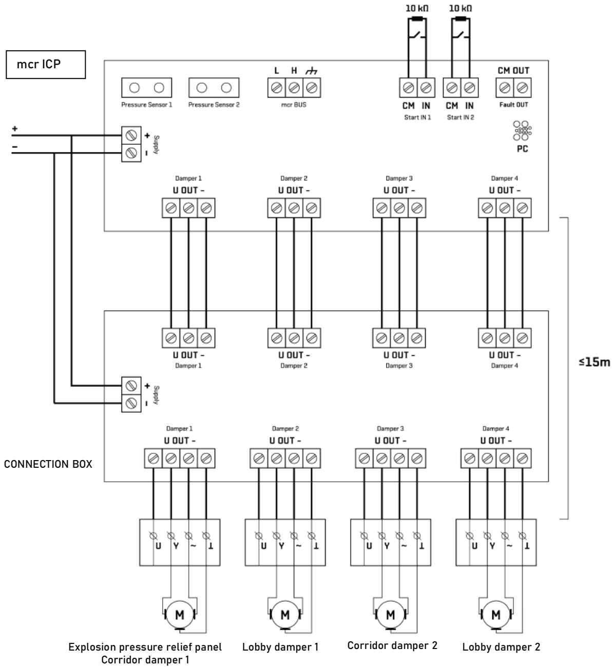
Figure 76 General block diagram for connecting mcr ICP and mcr PP regulators (support for 4 lobby dampers).
