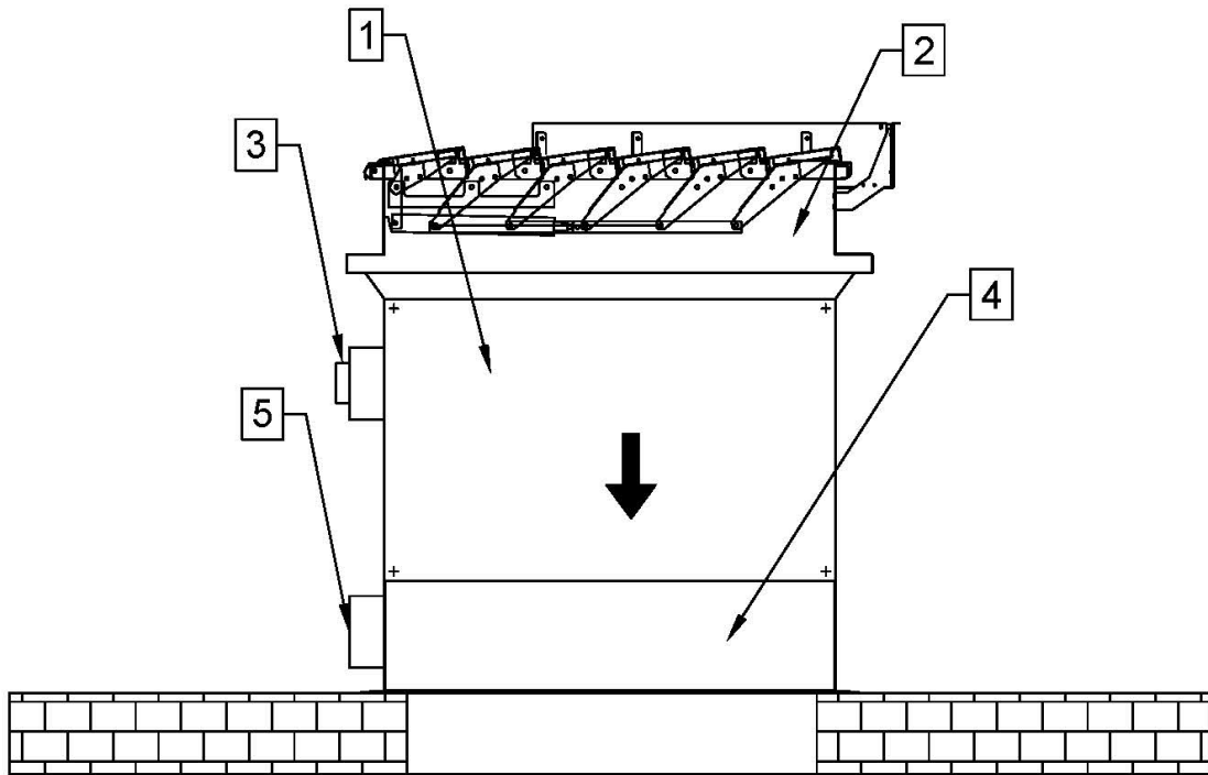
Figure 7 Sample installation of an air supply kit for the mcr EXi-F system in the UP version on the roof: 1 - fan, 2 - LAM vent with actuator, 3 - service disconnecter or connection box, 4 - roof base, 5 - duct smoke detector.
