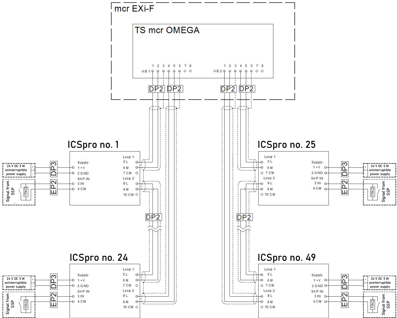
Figure 62 Block diagram for connecting mcr ICS Pro pressure transmitters in a lobby setup connected in two communication loops.
