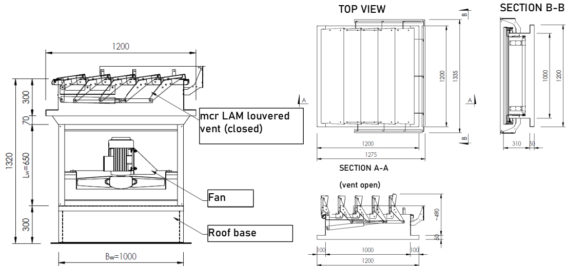
Figure 100. Vertical installation with louvered vent: mcr EXi-F 71-1S UP, 71-2S UP, 80-1S UP.
