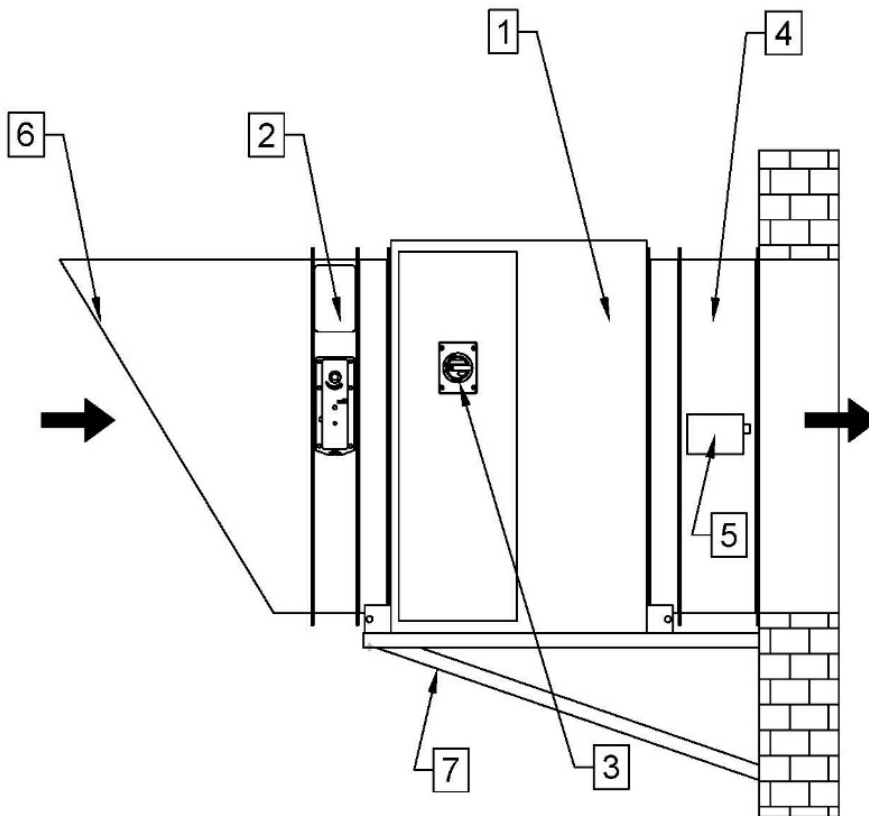
Figure 8 Sample installation of an air supply kit for the mcr EXi-F system in the wall-mounted version indoors: 1 - fan in a box-type housing, 2 - damper with actuator, 3 - service disconnecter or connection box, 4 - lead, 5 - duct smoke detector, 6 - inlet nozzle with grate, 7 - supporting structure.
