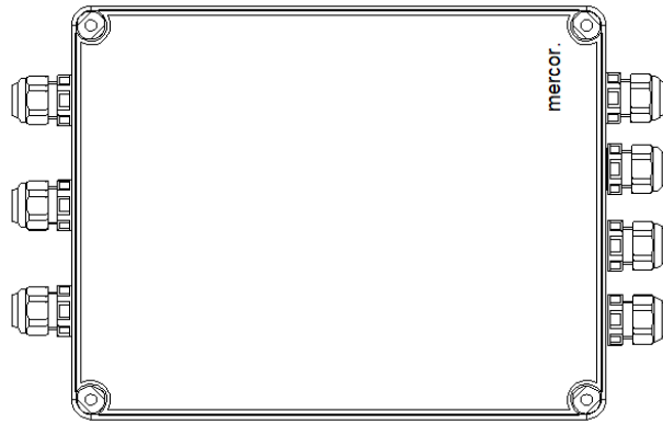
Figure 32 Overview of the mcr PP connection box (dimensions: without glands: 220 mm x 170 mm x 86 mm, with glands: 274 mm x 170 mm x 86 mm).
