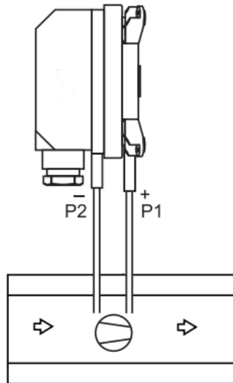
Figure 110 Installation diagram of a LF series differential pressure switch.
