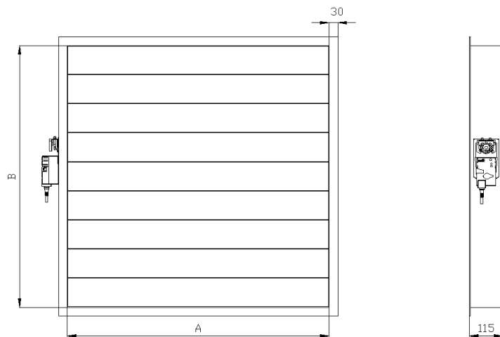
Figure 34 Overview of the EPSRC-A damper.
