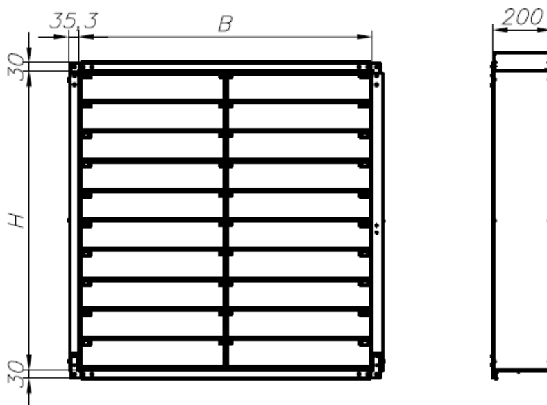
Figure 19 Overview of the PL explosion pressure relief panel.
