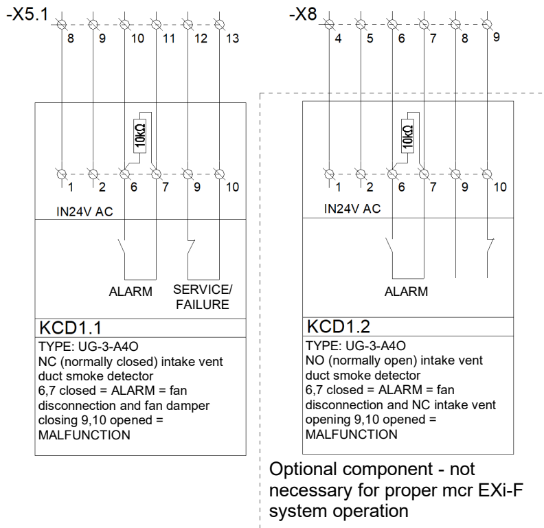
Figure 84 UG-3-A4 duct smoke detector connections circuit diagram.
