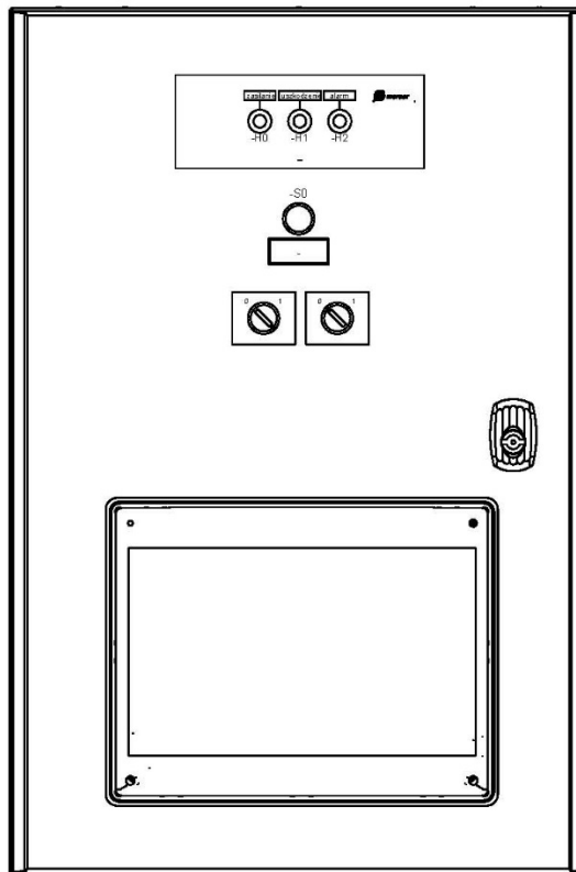
Figure 26 Overview of an elevated control panel with visualization.
