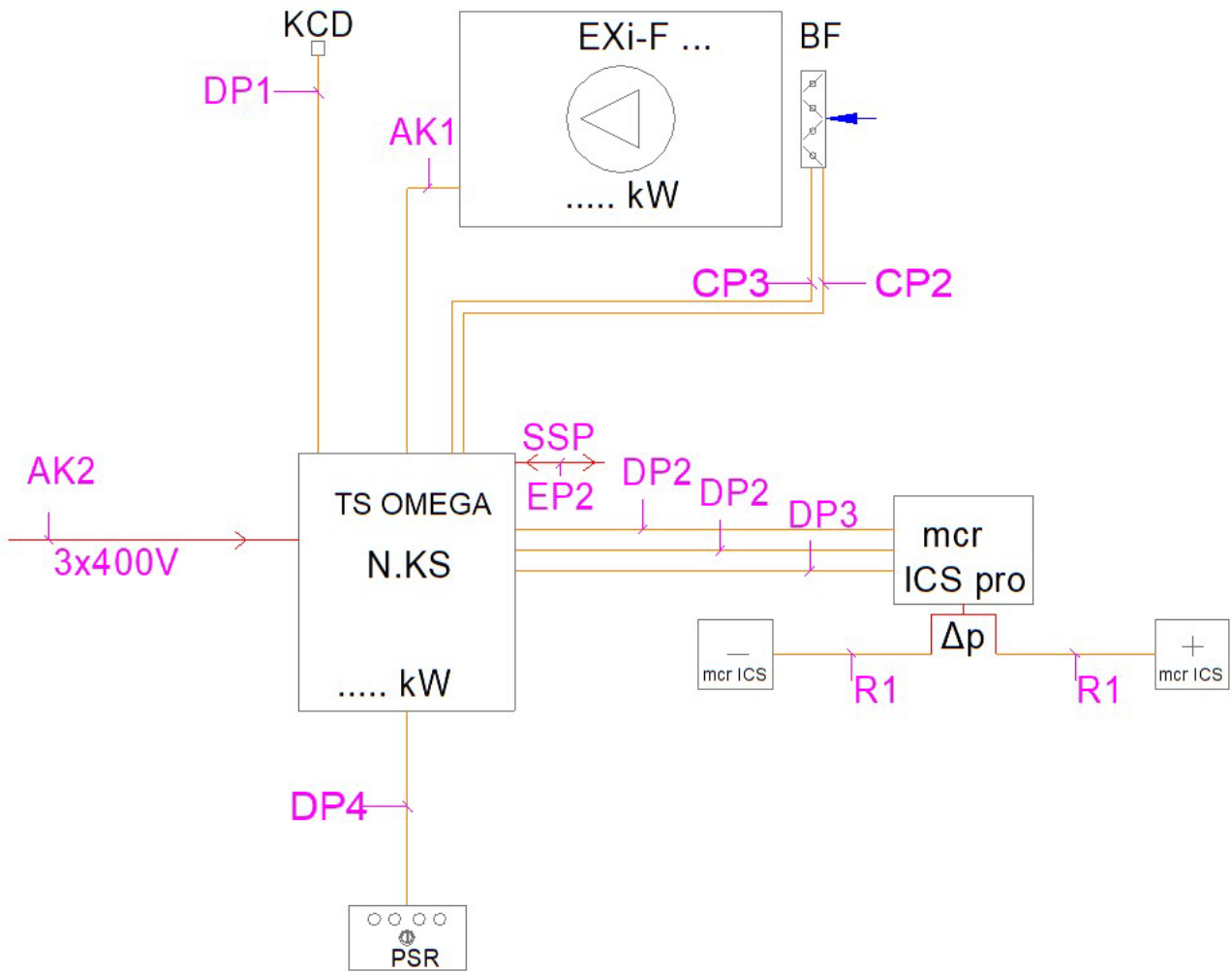
Figure 49 Schematic wiring diagram for a basic unit.
