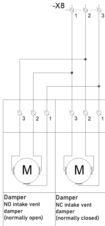
Figure 75 Connections circuit diagram for two dampers in the intake vent switching system.
