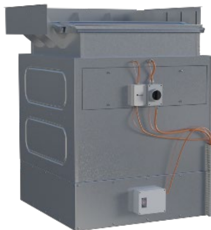
Figure 4 Design of the mcr mcr EXi-F air supply unit (UP vertical version).
