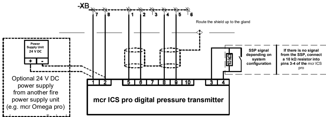
Figure 80 mcr ICS pro differential pressure transmitter connections circuit diagram
