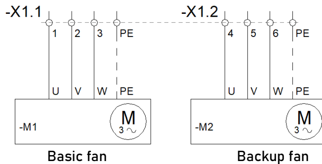
Figure 71 Fans connections circuit diagram.
