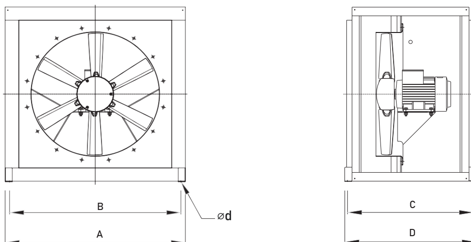
Figure 11 Installation dimensions of mcr EXi-F system air supply unit fans.
