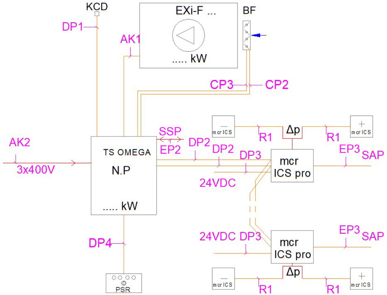
Figure 54 Schematic wiring diagram for lobby air supply.
