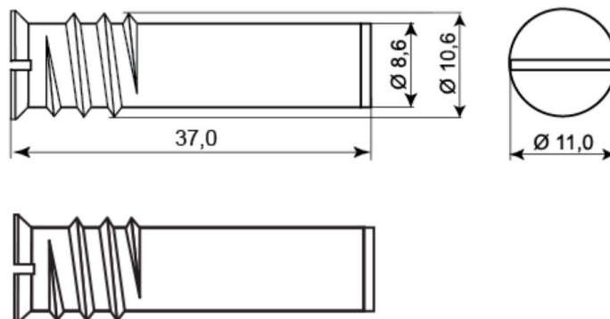
Figure 109 Installation dimensions of MC-240 series sensors.
