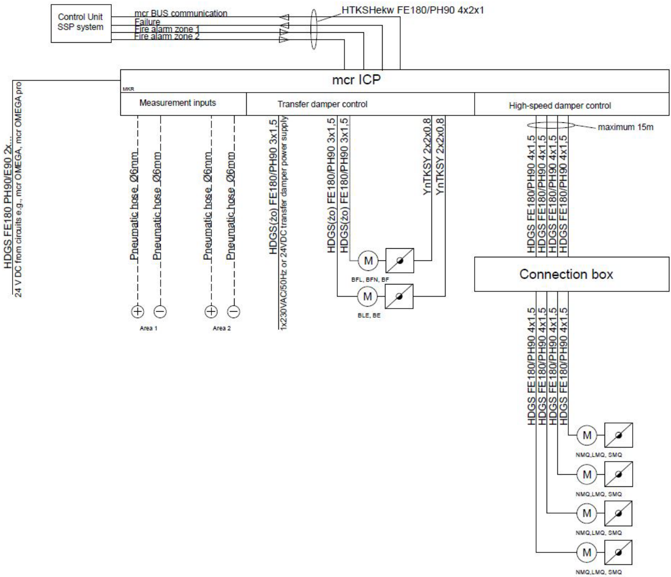
Figure 46 Electrical connection diagram for the mcr ICP lobby regulator handling 2 corridors and 4 high-speed dampers.
