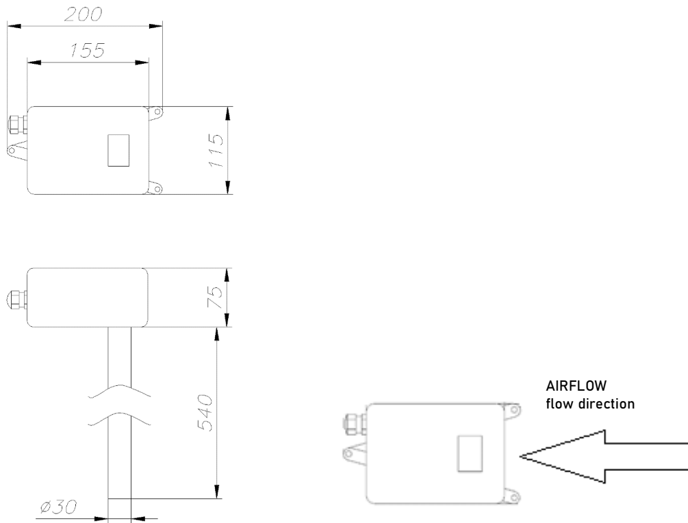
Figure 104 Installation rules along with dimensions of the SDD series sensor.
