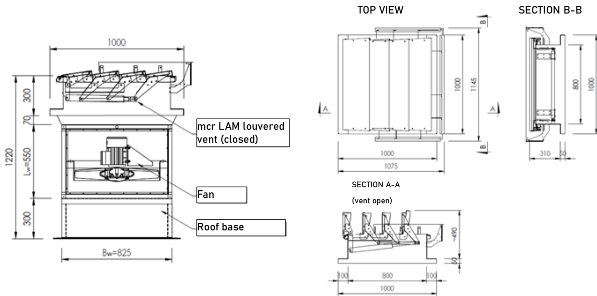
Figure 99 Vertical installation with louvered vent: mcr EXi-F 63- 1S UP.
