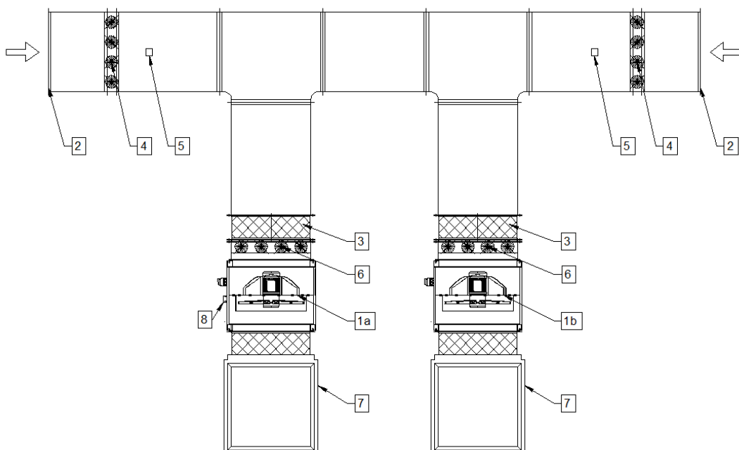
Figure 10 Sample installation of an mcr EXi-F air supply unit on the roof with a back-up unit: 1a - air supply unit basic fan, 1b - air supply unit back-up fan, 2 - intake vent, 3 - flexible connection, 4 - dampers with actuators in a double intake vent system, 5 - duct smoke detector, 6 - shut-off damper, 7 - ventilation duct, 8 - pressure switch.
