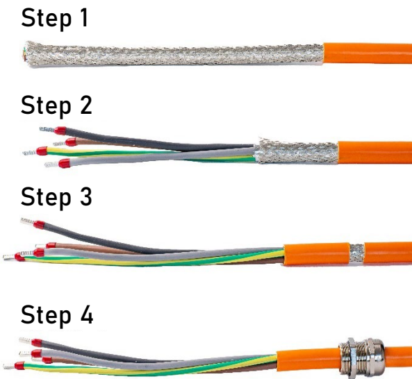
Figure 64 Step by step wire preparation guide.
