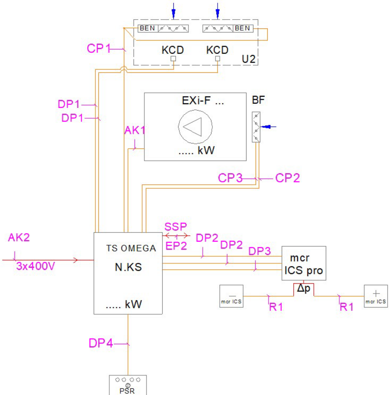
Figure 50 Schematic wiring diagram for a basic unit with a two intake vent system.
