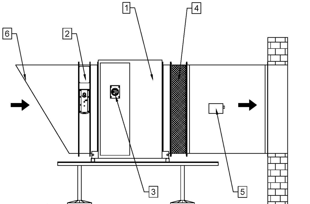
Figure 5 Sample installation of an air supply kit for the mcr EXi-F system: 1 - fan, 2 - damper with actuator, 3 - service disconnect or connection box, 4 - flexible connection, 5 duct smoke detector, 6 - inlet nozzle with grate.
