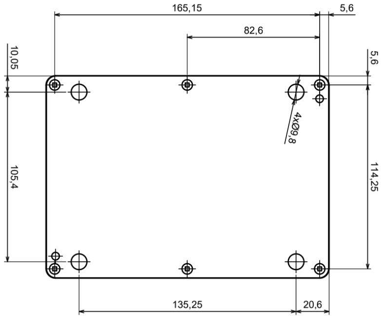
Figure 103 Dimensions of available mcr PSR/PRSC installation holes.
