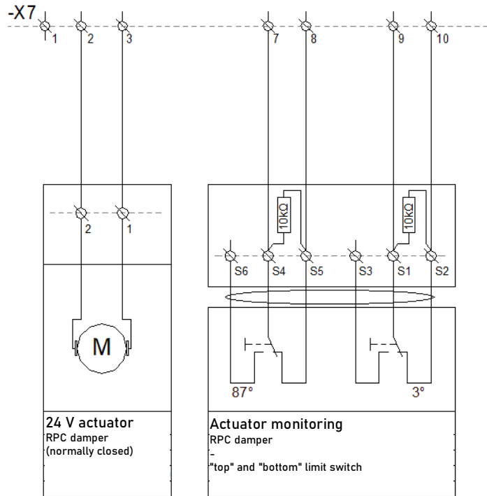
Figure 68 mcr RPC connections circuit diagram.
