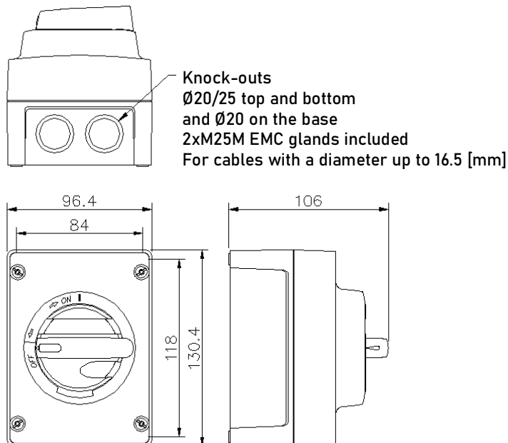
Figure 14 Overview of the service disconnecter.
