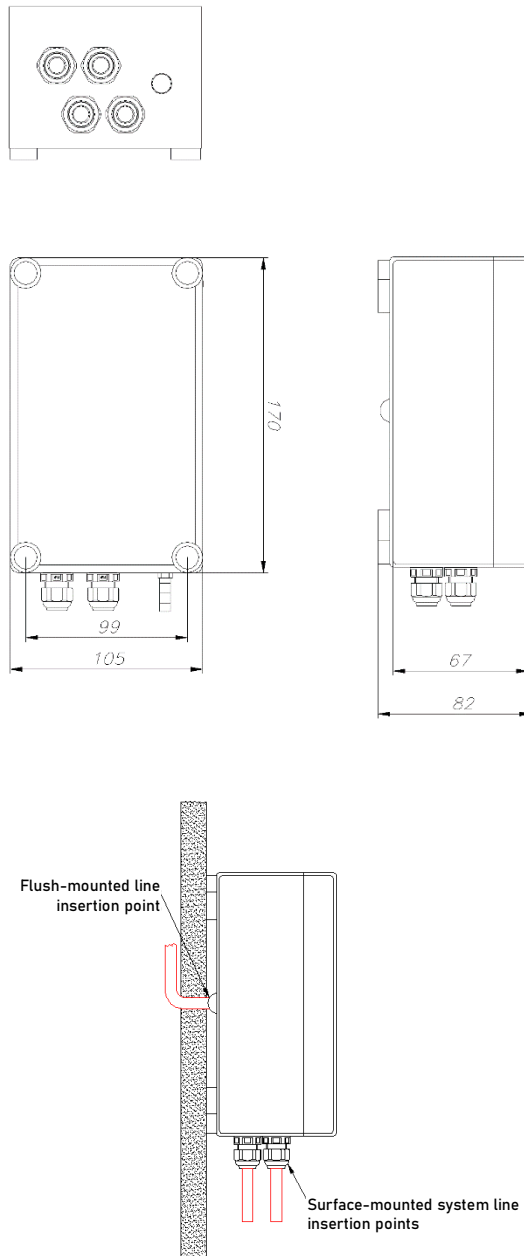
Figure 102 ICS pro transmitter installation dimensions.
