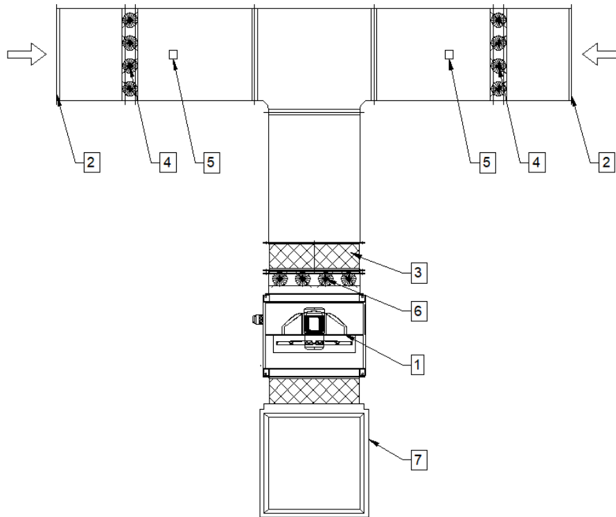
Figure 28 Sample installation of an air supply kit for the mcr EXi-F system in the roof-mounted version with two air intake vents: 1 - fan, 2 - intake vent, 3 - flexible connection, 4 - dampers with actuators in a double intake vent system, 5 - duct smoke detector, 6 - shut-off damper, 7 - ventilation duct.
