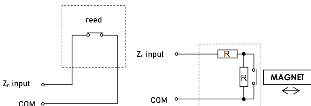
Figure 42 Manners of connecting magnetic sensors (reeds).
