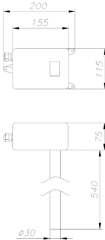
Figure 27 SDD-65-RAC duct smoke detector - overview.
