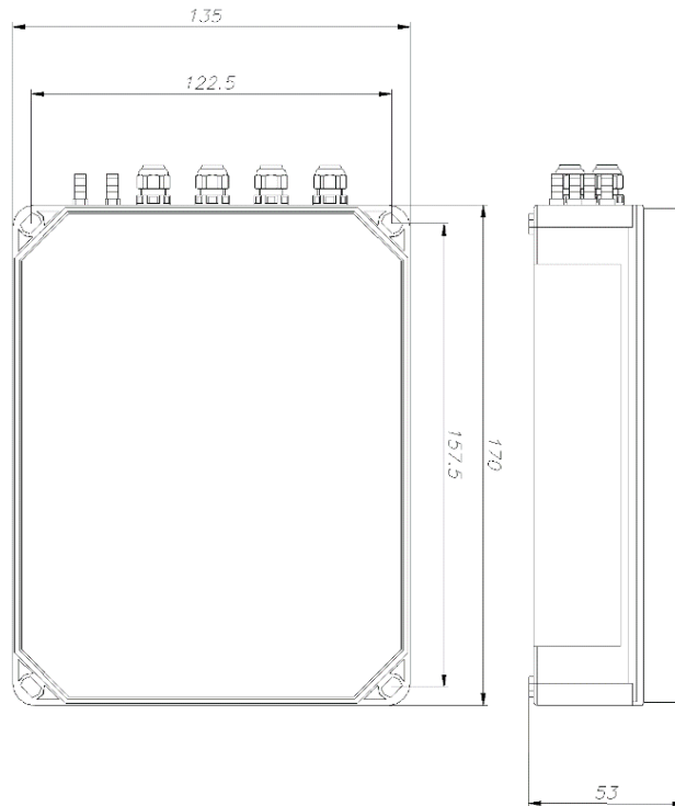
Figure 105 Dimensions of mcr ICP regulator installation holes.
