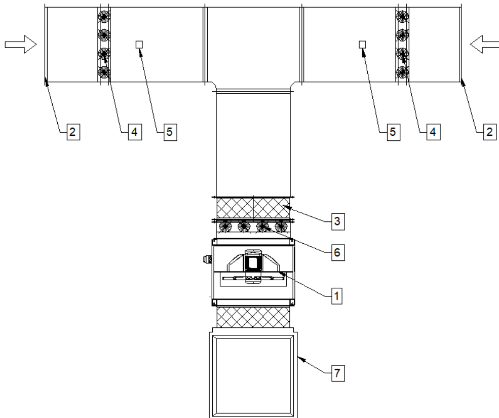
Figure 9 Sample installation of an air supply kit for the mcr EXi-F system in the roof-mounted version with a double air intake vent system: 1 - fan, 2 - intake vent, 3 - flexible connection, 4 - dampers with actuators in a double intake vent system, 5 - duct smoke detector, 6 - shut-off damper, 7 - ventilation duct.
