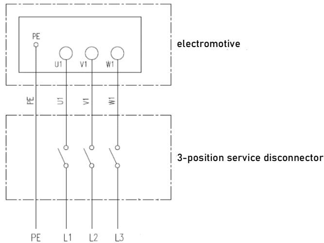
Figure 65 Electrical diagram of the service disconnector for the air supply unit fan.
