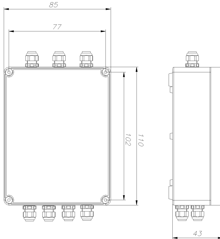
Figure 106 Dimensions of mcr PP connection box installation holes.
