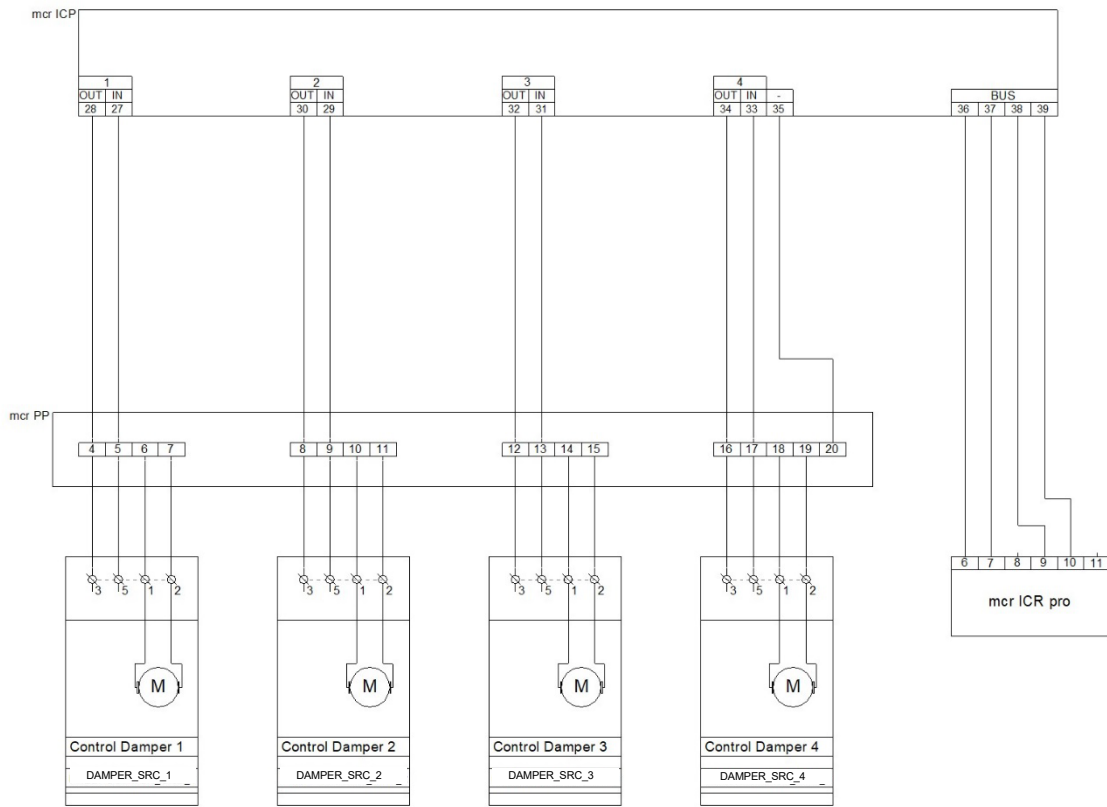
Figure 77 Block diagram for connecting a mcr ICP regulator in the communications network with mcr Omega.
