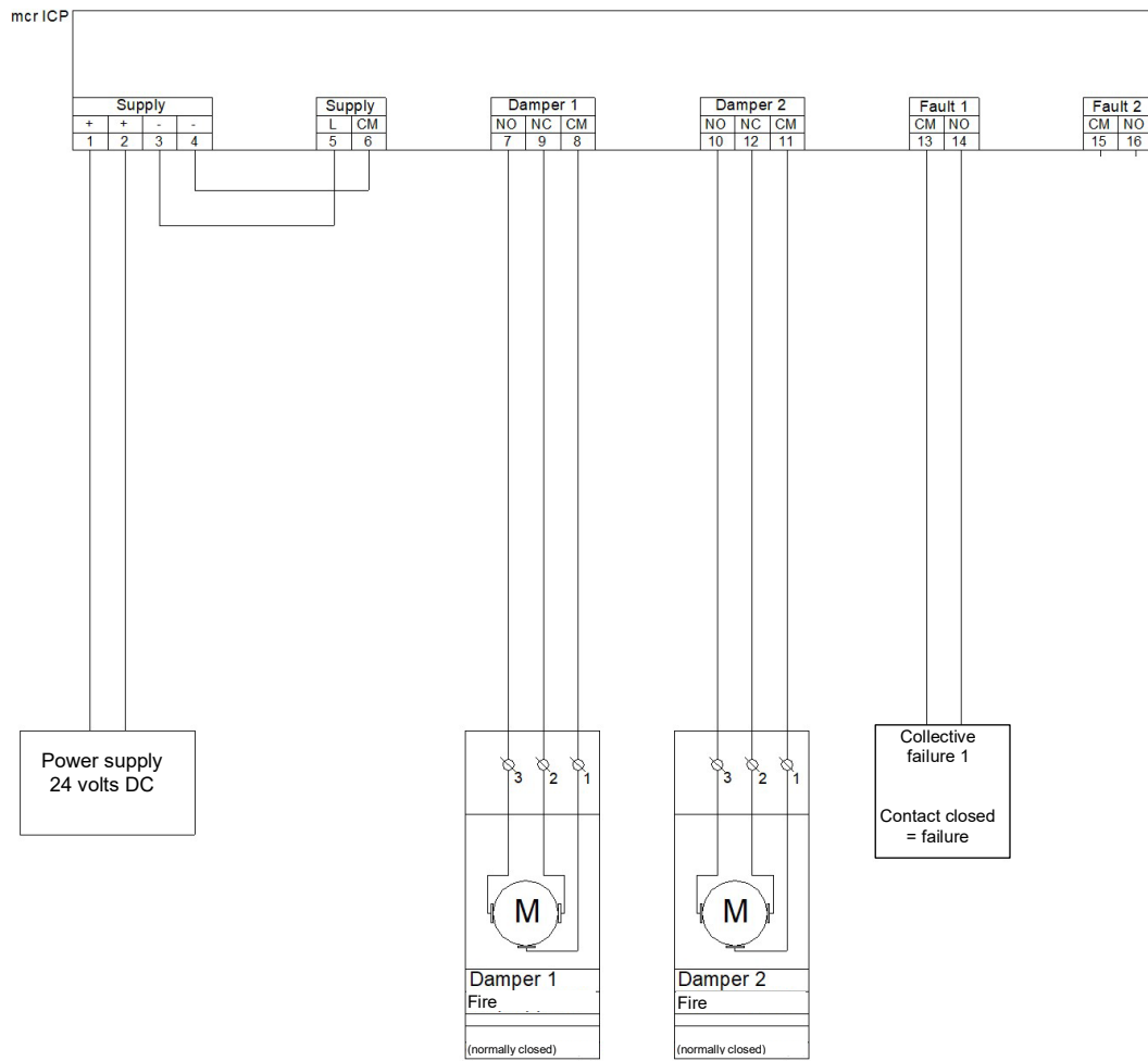
Figure 78 Block diagram for connecting a mcr ICP regulator – option with support for fire ventilation vents.
