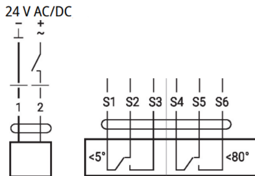
Figure 87 Connections circuit diagram for the Belimo BF/BFL/BFN series actuator. Actuators used in shut-off dampers at mcr EXi-F air supply units.
