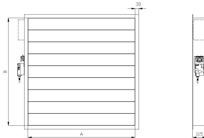
Figure 35 Overview of the EPSRC-B 9 damper (with additional connection box).
