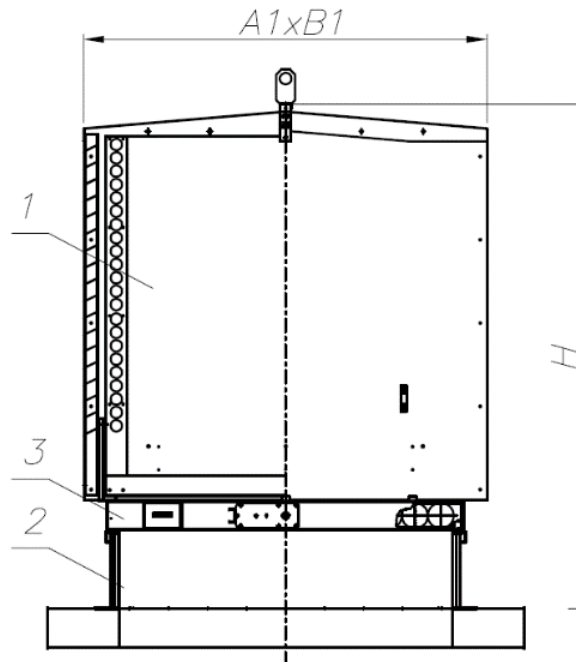
Figure 20 Overview of the PLD explosion pressure relief panel: 1 - vent, 2 - base, 3 - damper with actuator.
