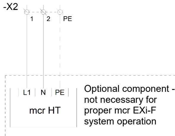
Figure 86 Electrical connection of the mcr Omega panel for the anti-icing system.
