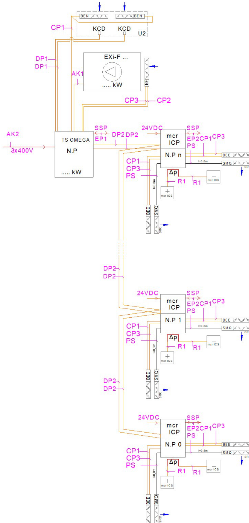
Figure 55 Schematic wiring diagram for a unit with high-speed mcr ICP dampers secured with smoke control system vents.
