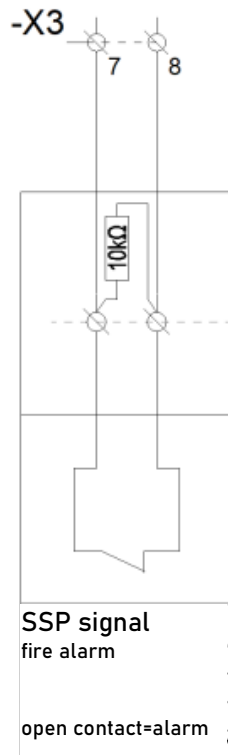
Figure 69 Connection of SSP signal (fire ALARM) to the EXi-F panel.
