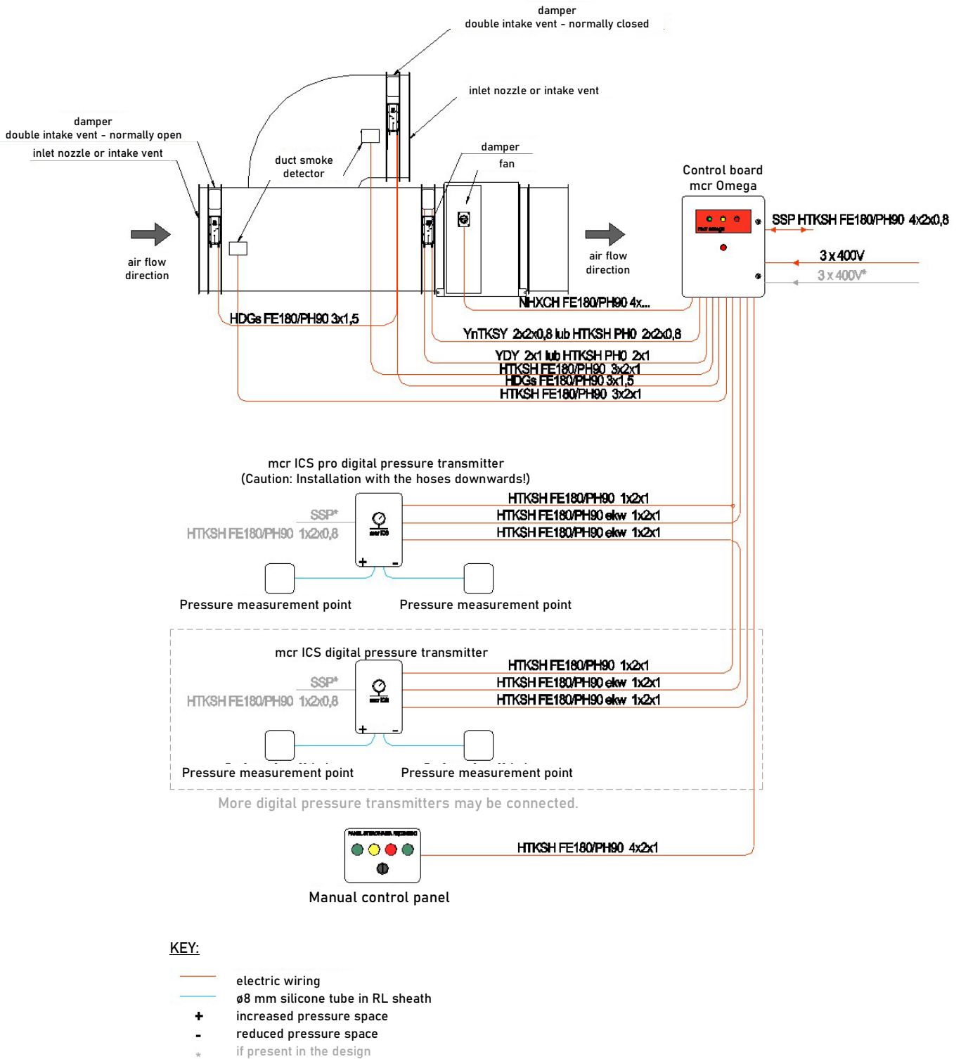
Figure 48 Wiring of the EXi-F unit with a two intake vent system.
