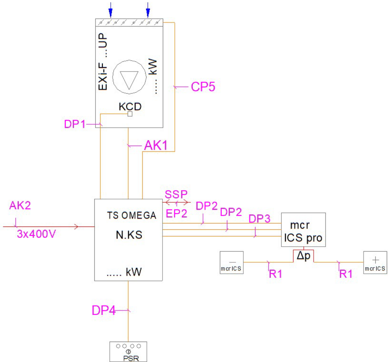
Figure 53 Schematic diagram of a vertical unit with a mcr LAM vent.
