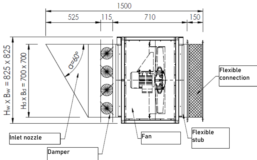
Figure 96 Basic dimensions of the standard mcr EXi-F 63-1 air supply units in a box-type housing - horizontal installation.
