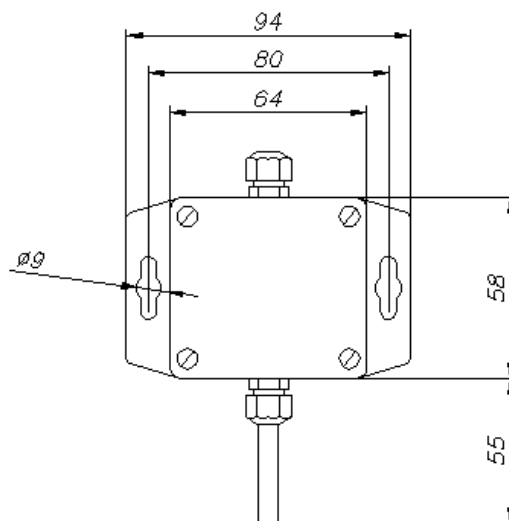
Figure 41 Overview for the AR series temperature transmitter.
