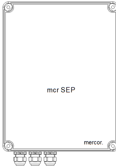
Figure 38 Overview of mcr SEP network separator (dimensions: without glands: 220 mm x 170 mm x 86 mm, with glands: 247 mm x 170 mm x 86 mm).
