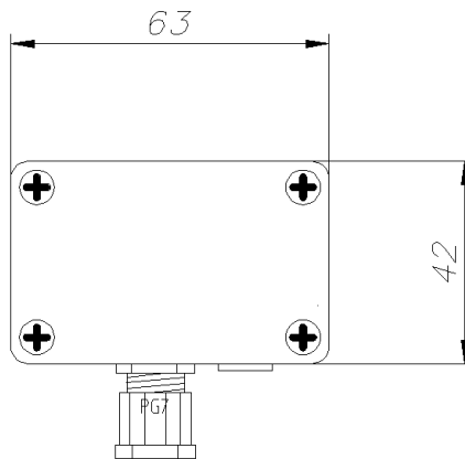
Figure 40 Overview and connection details for the MB series temperature transmitter.
