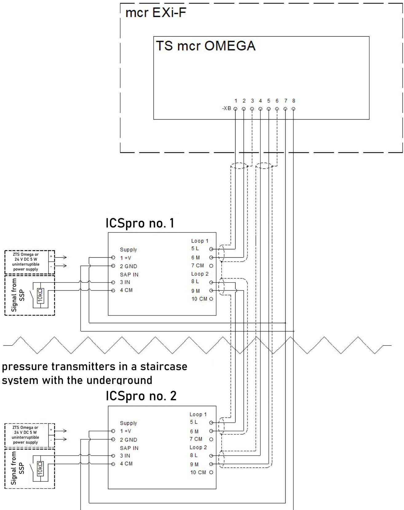
Figure 60 Block diagram for connecting mcr ICS Pro pressure transmitters in a staircase system with separate transmitters in the underground part triggered from the FSS.
