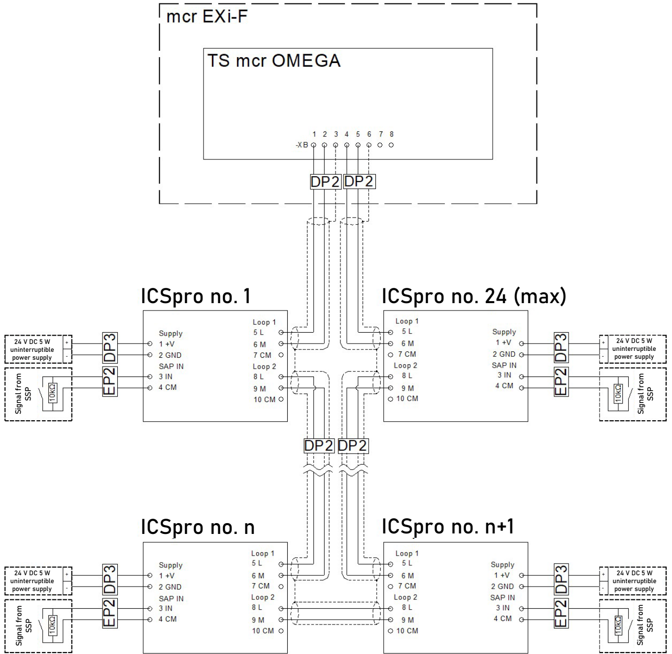
Figure 61 Block diagram for connecting mcr ICS Pro pressure transmitters in a lobby setup.
