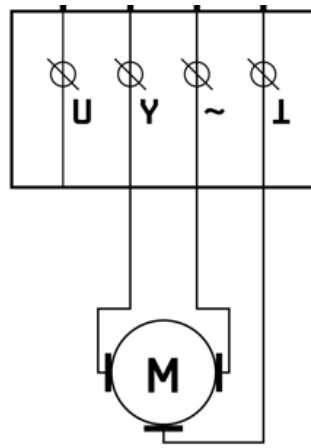
Figure 30 Connections circuit diagram for the Belimo NMQ/LMQ/SMQ series actuator.
