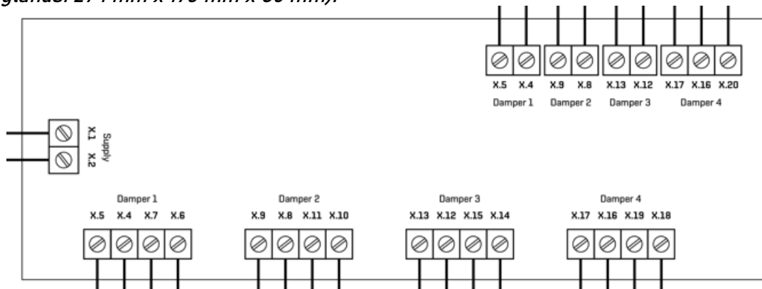
Figure 33 Terminals in the mcr PP box.
