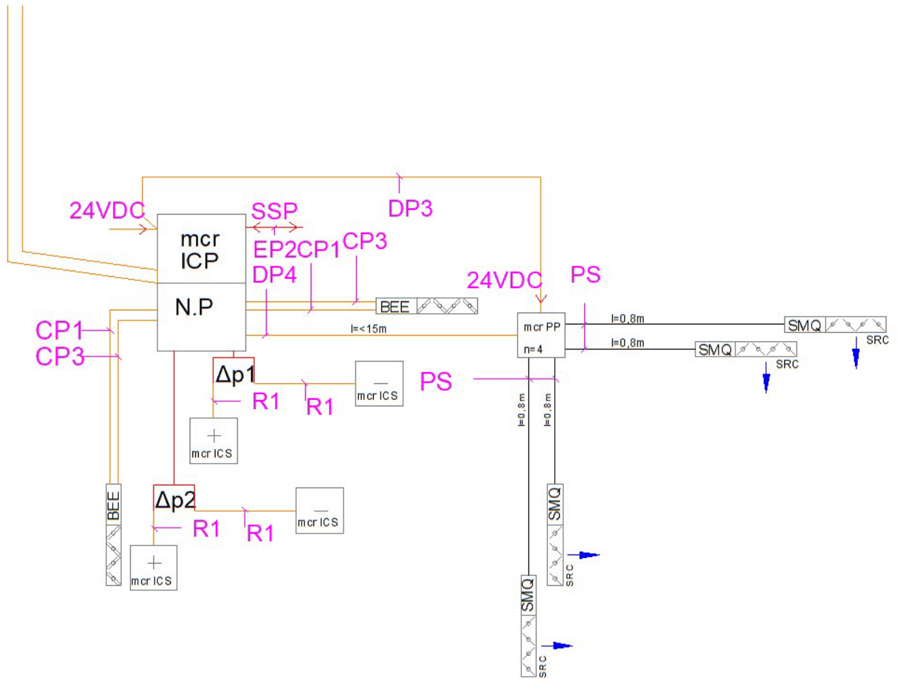
Figure 57 Schematic diagram for connecting four high-speed dampers to the mcr ICP high-speed damper regulator through a mcr PP box.
