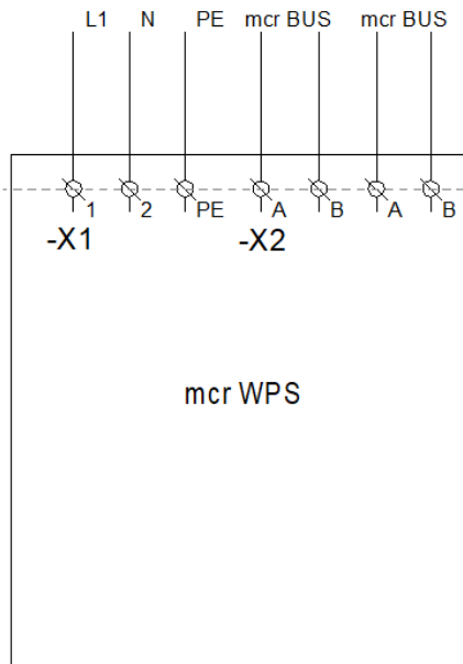
Figure 83 Electrical connection of the mcr WPS panel (U=230 V AC).
