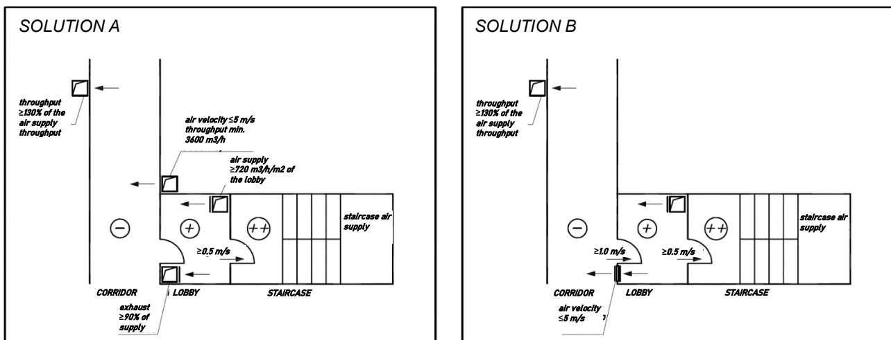
Figure 2 Design requirements diagram for solutions A and B.
