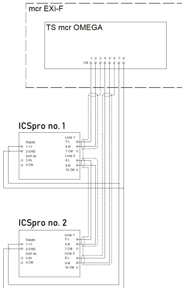
Figure 59 Block diagram for connecting mcr ICS Pro pressure transmitters in a staircase-two transmitters setup.
