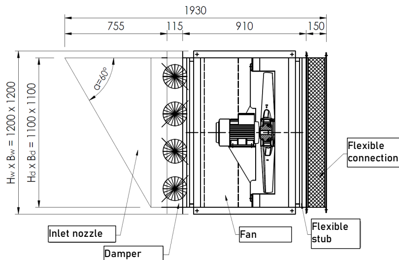
Figure 98 Basic dimensions of the standard mcr EXi-F 90-1S, 90-2S, 100-1S, 100-2S air supply units in a box-type housing - horizontal installation.
