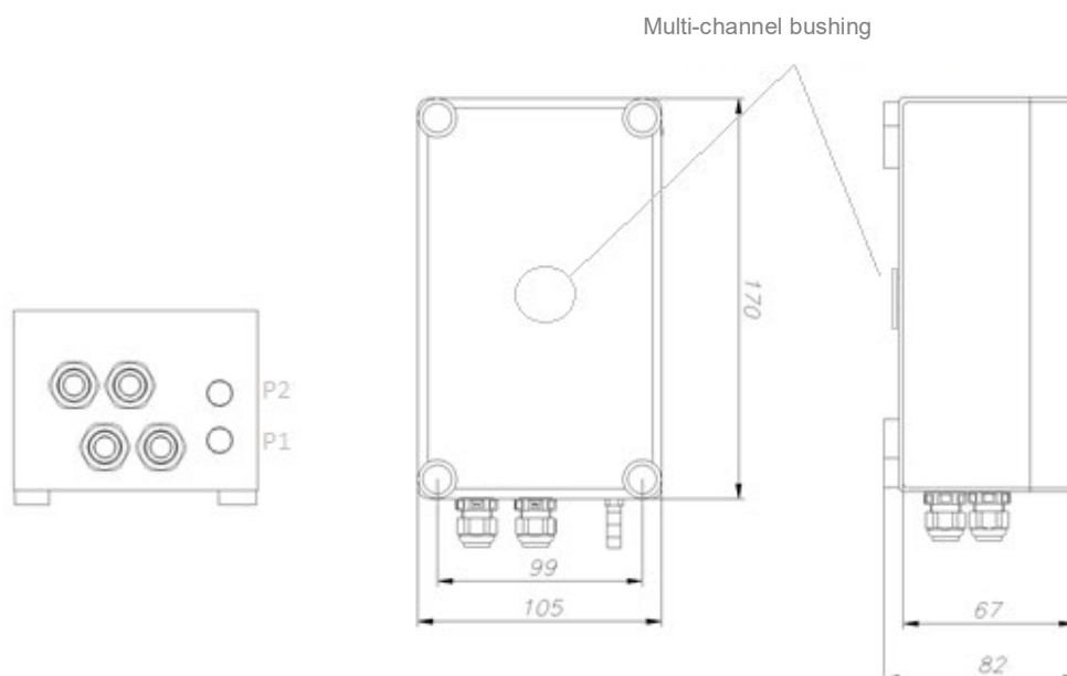
Figure 23 mcr ICS pro digital pressure transmitter - overview.
