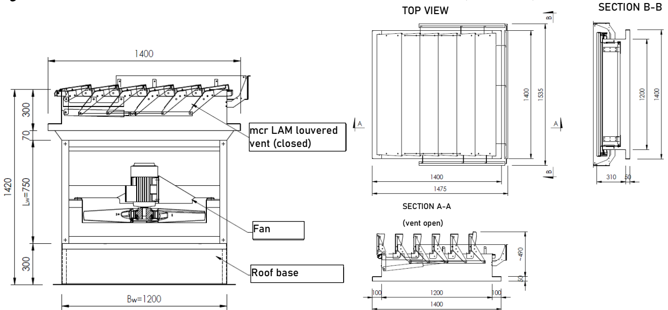
Figure 101 Vertical installation with louvered vent: mcr EXi-F 90-1S UP,90-2S UP,100-1S UP,100-2 S UP.
