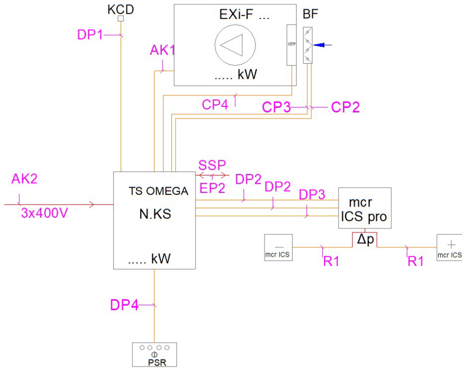
Figure 51 Schematic wiring diagram for a unit with the mcr HT anti-icing system.
