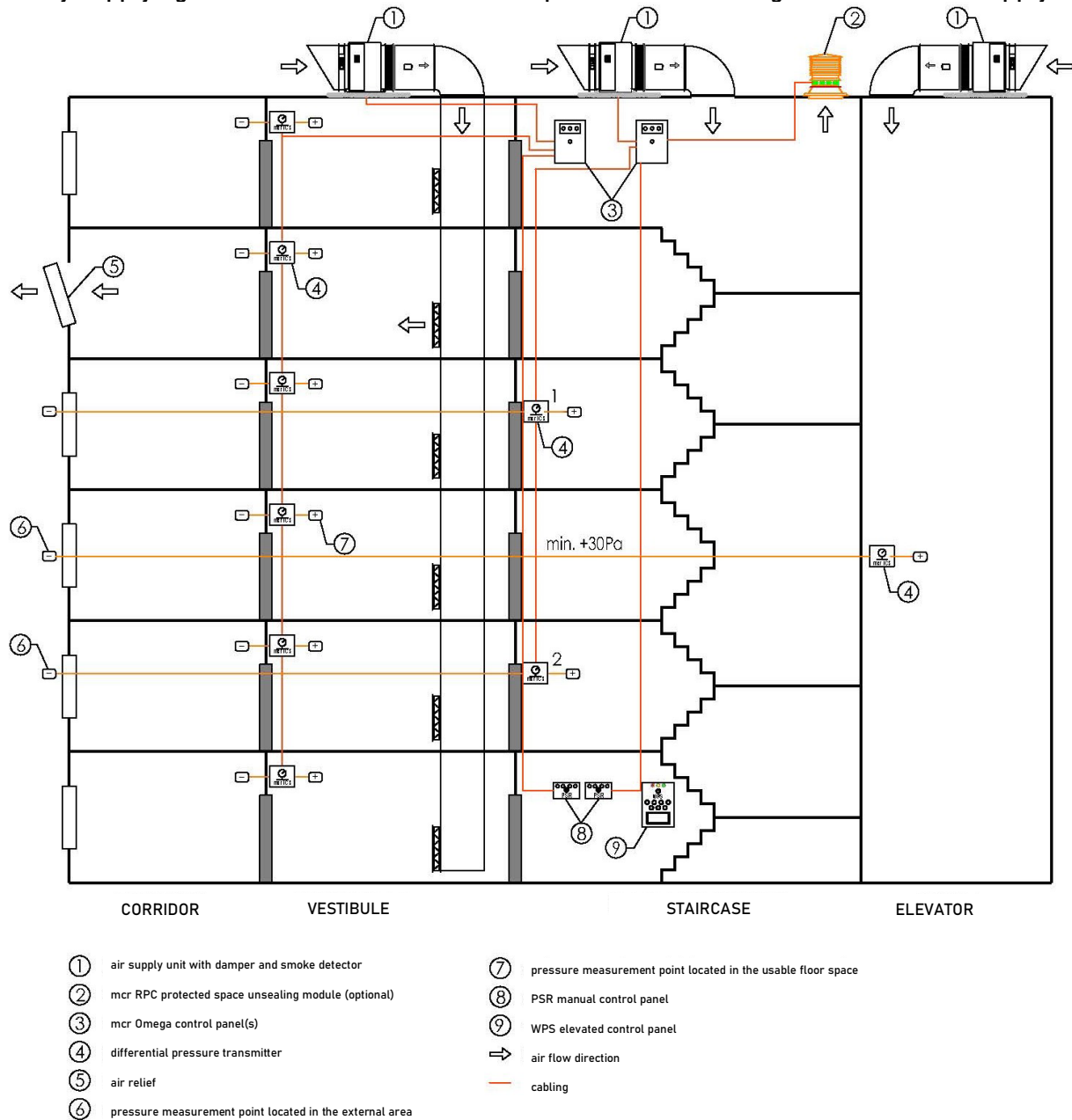
Figure 1 mcr EXi-F system schematic diagram.
