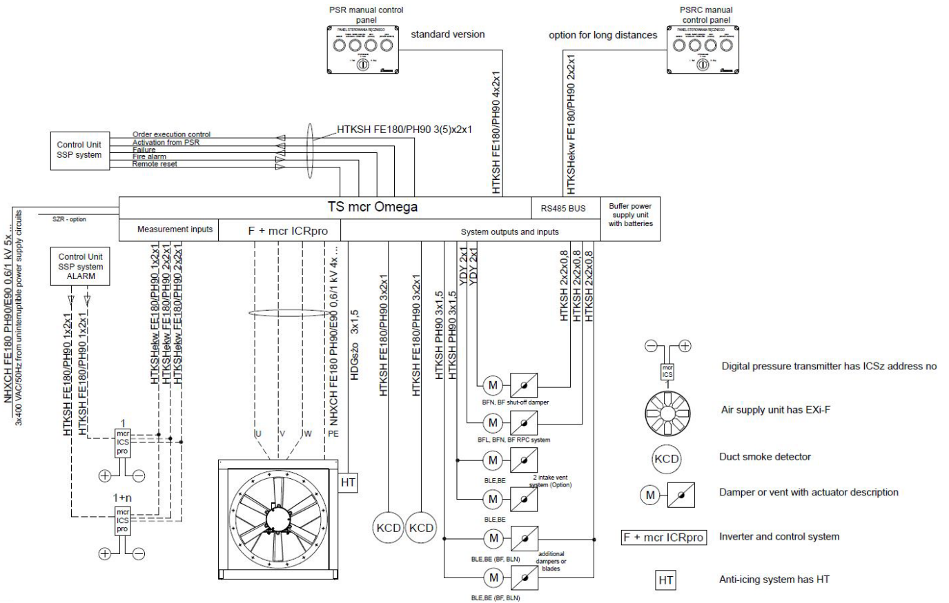
Figure 45 General electrical connection diagram for the EXi-F system: electrical connection, suggested types of wires for the mcr Omega control panel.
