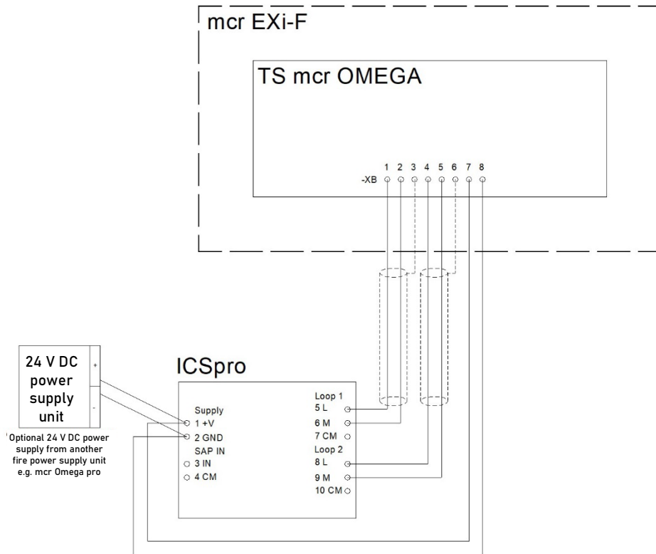
Figure 58 Block diagram for connecting a mcr ICS Pro pressure transmitter in a staircase-single transmitter setup.
