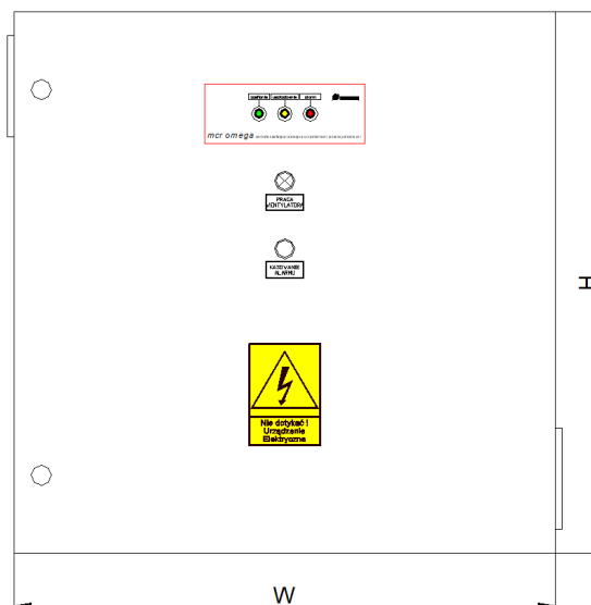
Figure 22 mcr Omega control panel overview.
