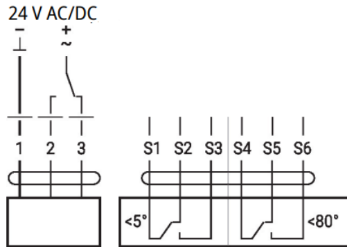
Figure 88 Connections circuit diagram for the Belimo BE/BEE/BLE series actuator. Actuators used in dampers in double intake vent systems.
