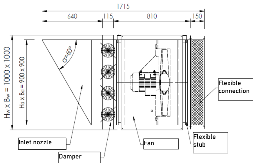
Figure 97 Basic dimensions of the standard mcr EXi-F 80-1S, 71-1S, 71-2S air supply units in a box-type housing - horizontal installation.
