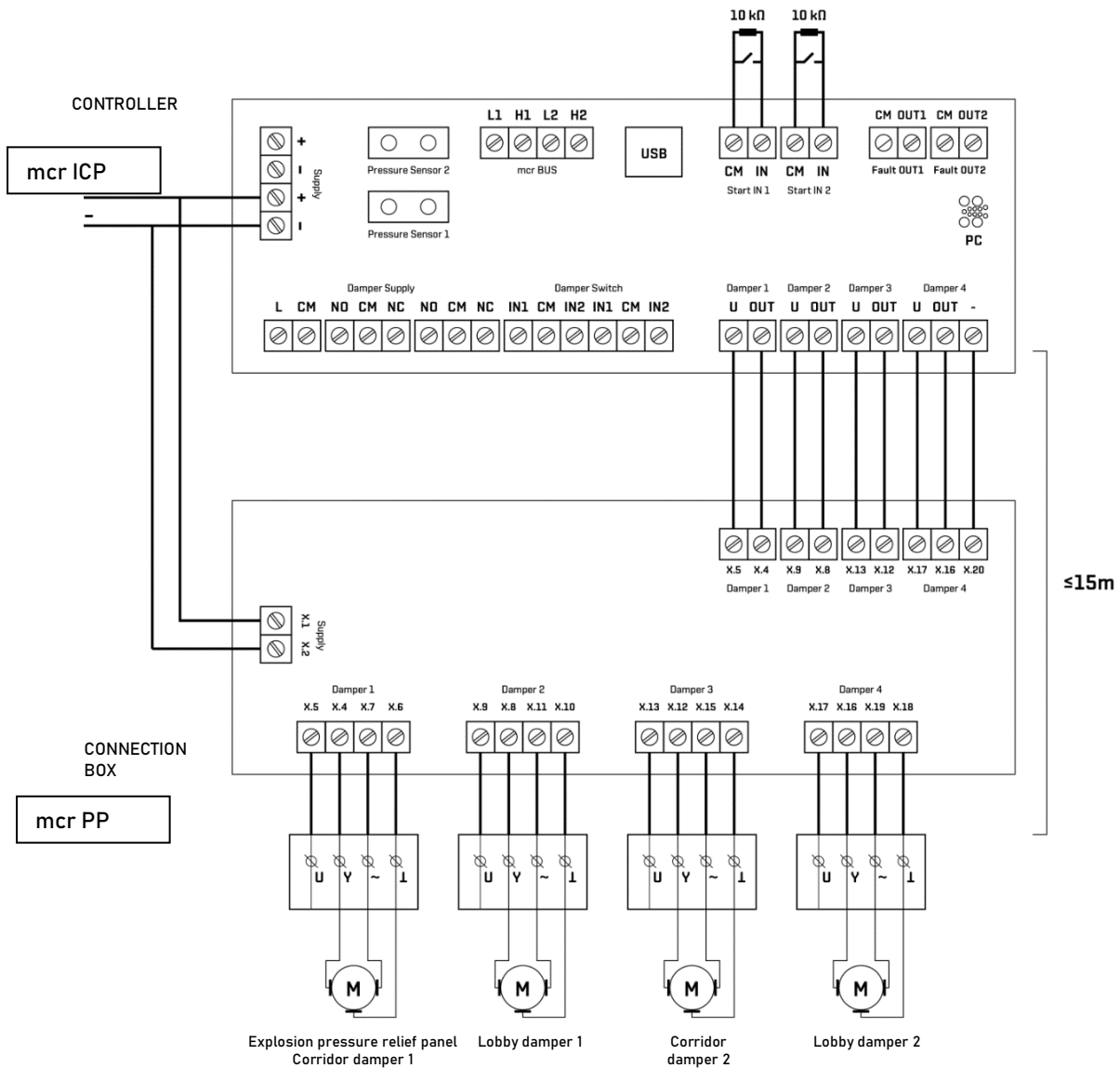
Figure 31 Connection of actuators to the mcr ICP regulator through the mcr PP connection box.
