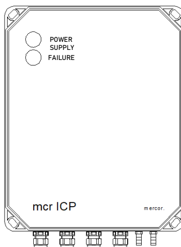
Figure 29 mcr ICP regulator overview (dimensions - Without glands and controls: 340 mm x 270 mm x 106 mm, with glands and indicator lights: 367 mm x 270 mm x 120 mm).
