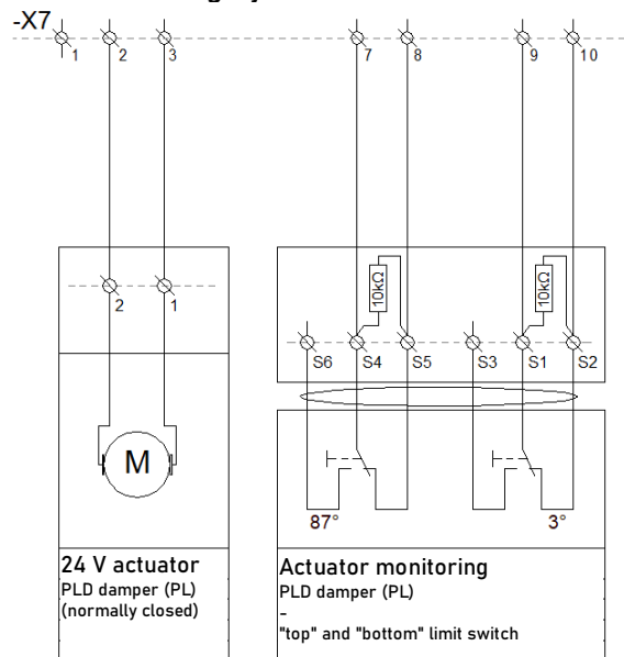
Figure 67 Connections circuit diagram for the Belimo BF, BFL, BFN series actuator.
