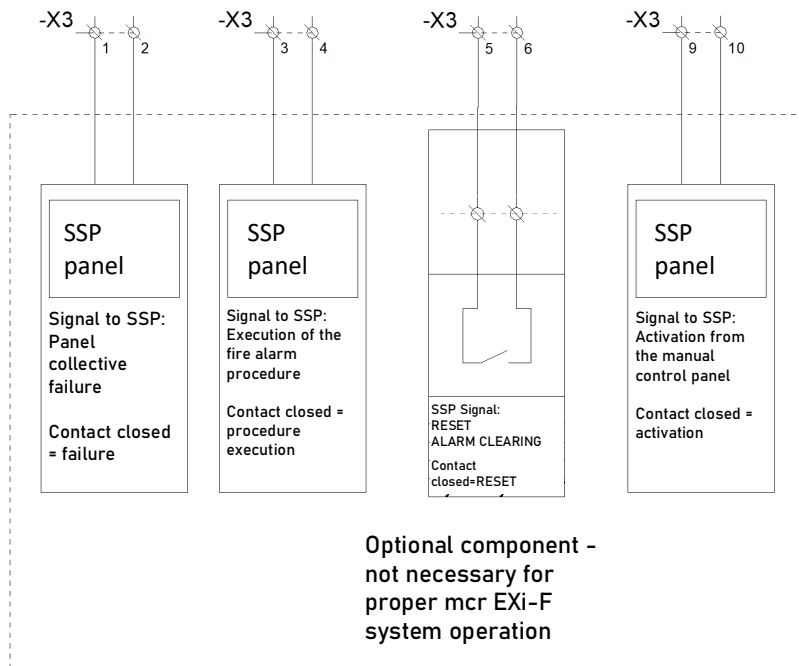
Figure 70 Connecting optional SSP signals to the mcr Omega panel.
