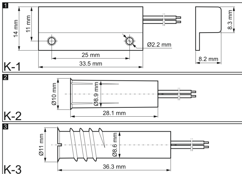
Figure 108 K-x series sensor installation dimensions.
