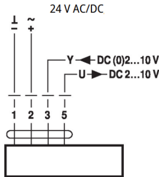
Figure 89 Connections circuit diagram for the Belimo NMQ/LMQ/SMQ series actuator.
