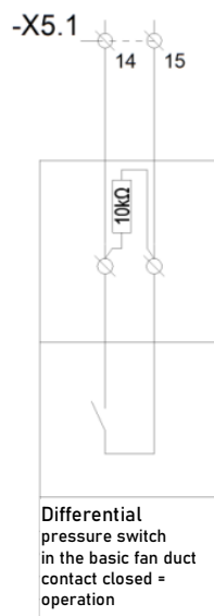
Figure 72 Pressure switch connections circuit diagram.
