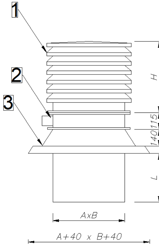
Figure 21 Detailed view of the RPC protected space unsealing module. 1. exhaust vent, 2 damper with BFN actuator, 3 roof base.
