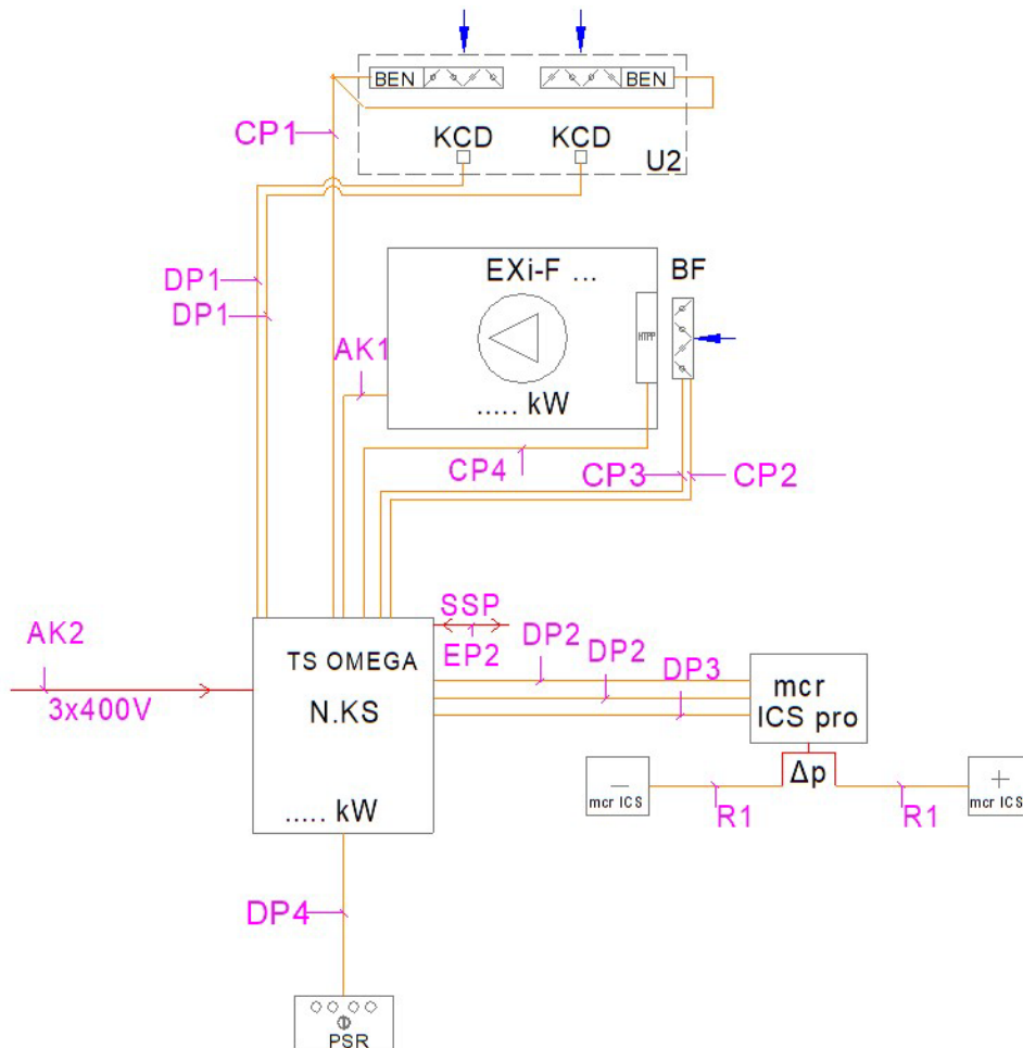
Figure 52 Schematic wiring diagram for a unit with a double intake vent system and mcr HT anti-icing system.
