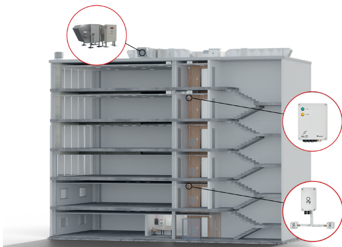
Fig. 7: Securing fire-fighting lobbies.
