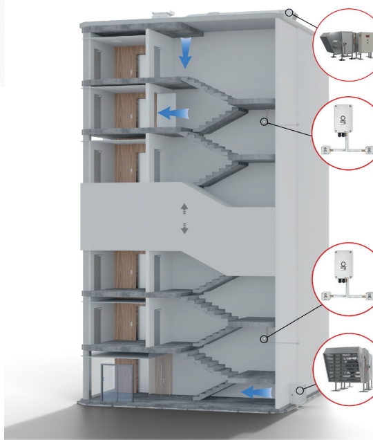
Fig. 3: In tall and high-rise buildings , where multi-point air supply using a duct is impossible, this requirement can be met by installing a sufficient number of air supply units. Each of the mcr EXi-F units protects a given staircase zone based on pressure readings from the differential pressure transmitter located in that zone. The system operation is controlled by dedicated mcr Omega control panels.
