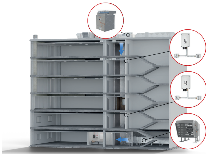
Fig. 6: Fire lifts.
