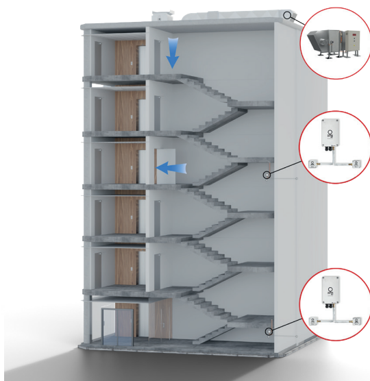
Fig. 2: In tall buildings , where the value of pressures in the lower and upper part of the staircase may be different, two pressure sensors should be used, together with one mcr EXi-F air supply unit. The algorithm implemented in the controller manages, through the actuators of the mcr Omega control panel, the speed of the air supply fan, controlling the average pressure value, as well as the minimum and maximum values that were determined during the system configuration.
