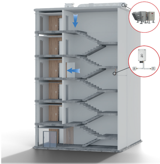
Fig. 1: In low-rise buildings , we use one mcr EXiF air supply unit along with one pressure sensor to protect staircases from smoke. An mcr PP pressure measurement point should be placed in the middle part of the staircase, avoiding the direct impact of the supplied air stream. The measurement reference point should be placed outside the building. The system operation is controlled by a dedicated mcr Omega control panel.
